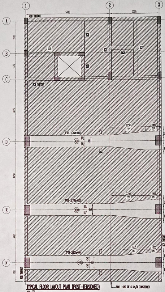
TYPICAL-2ND FLOOR
