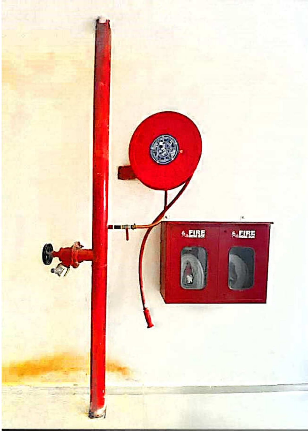
A typical picture showing Downcomer, Hose reel drum & Fire hose box (double door) installed at site.
