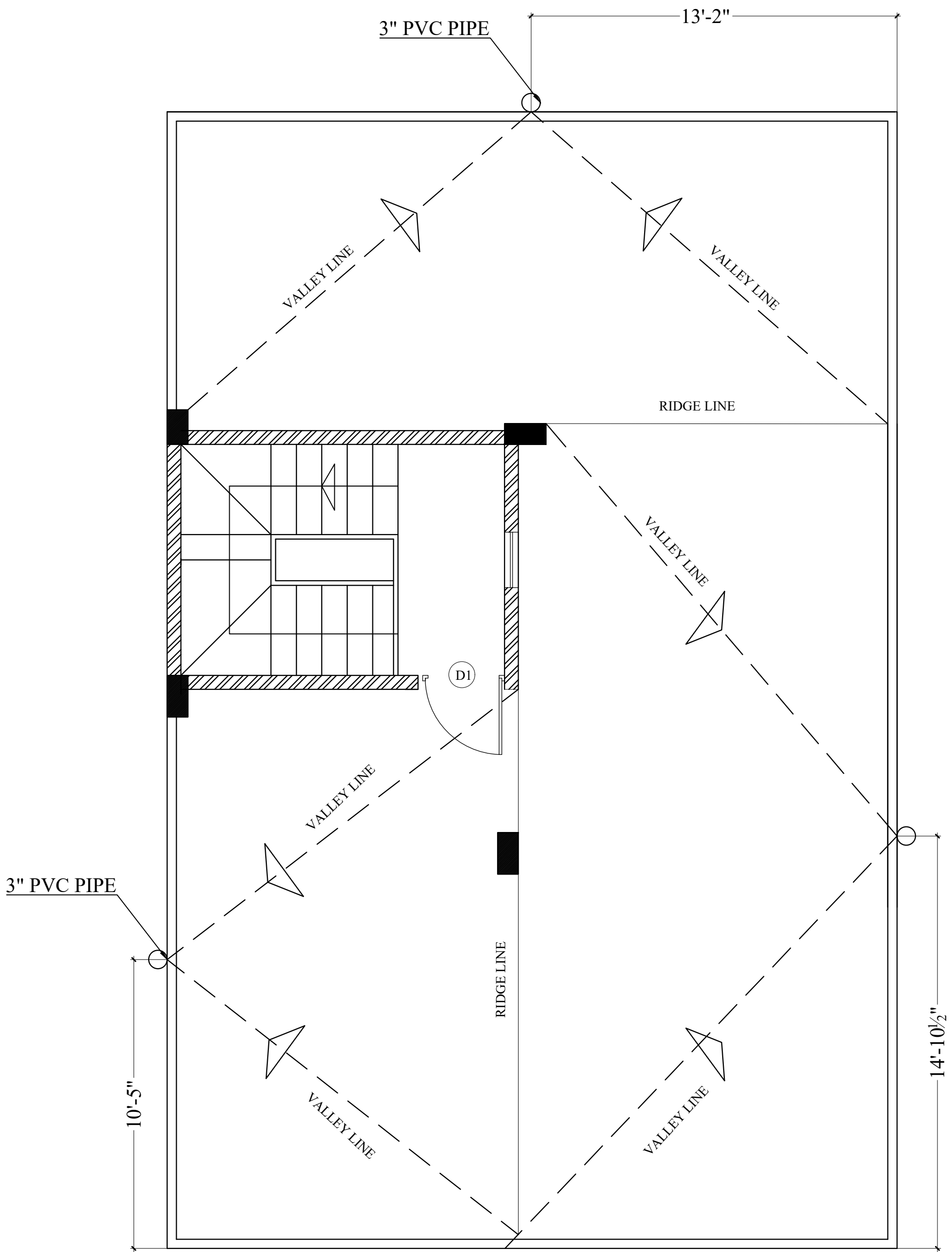
A1 (3BHK) - ROOF FLOOR PLAN
