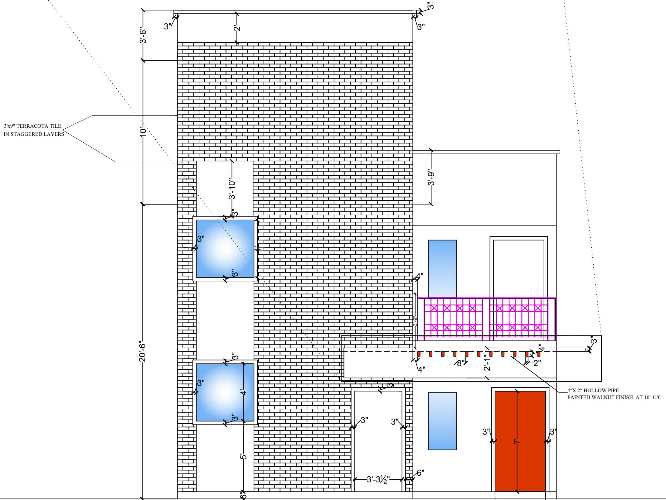
FRONT ELEVATION
