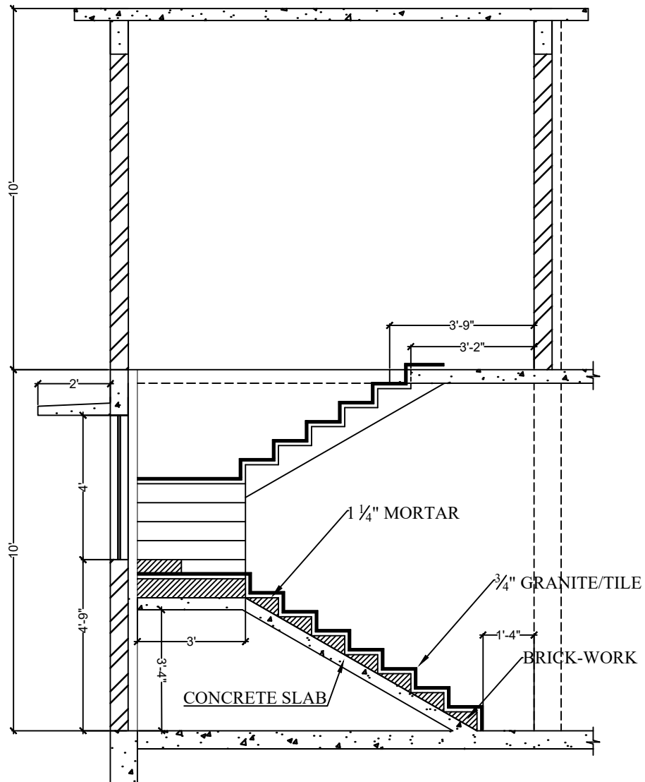
SECTION @ B-B'
