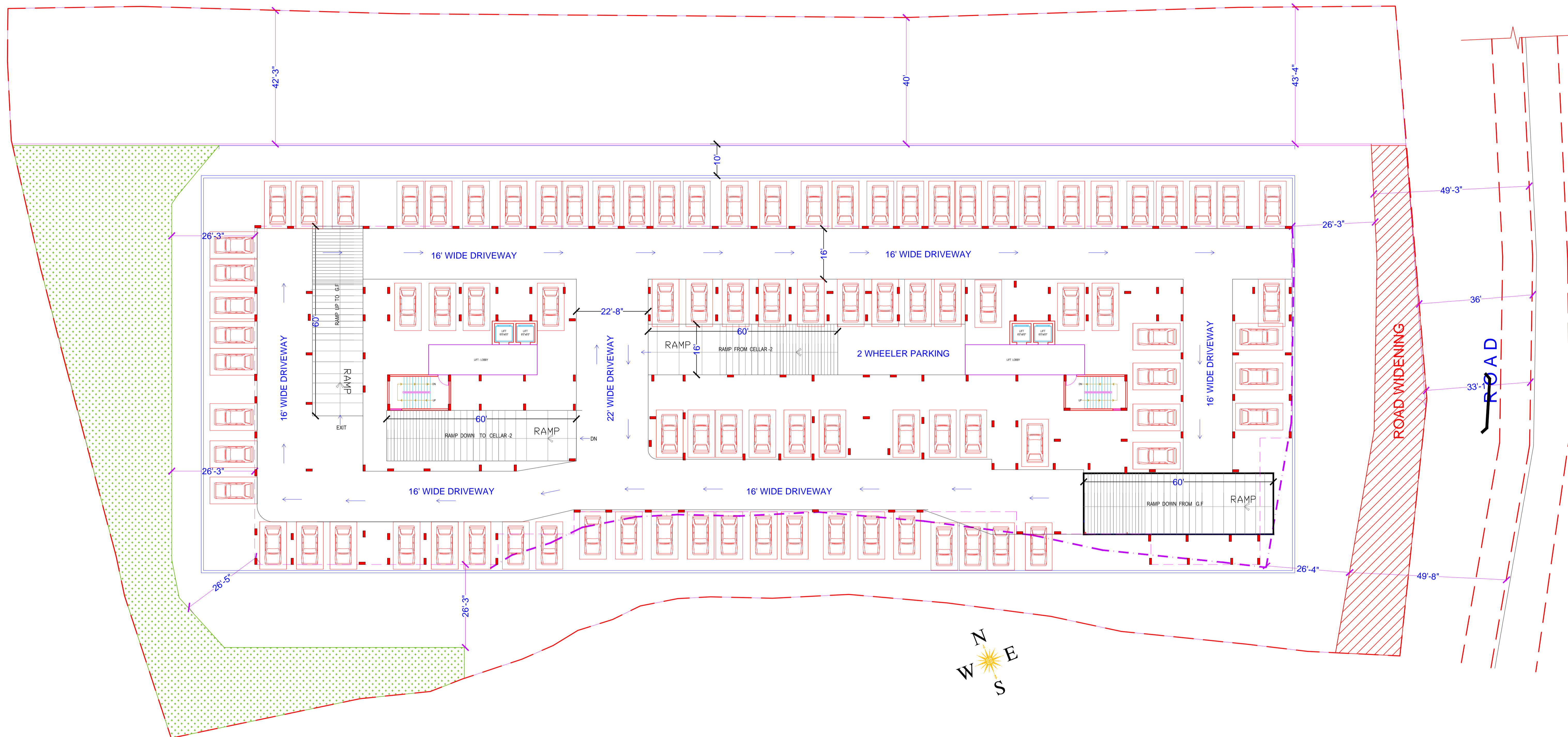
FLOOR PLAN - CELLAR-1 TOTAL Nos. of CARS - 207
