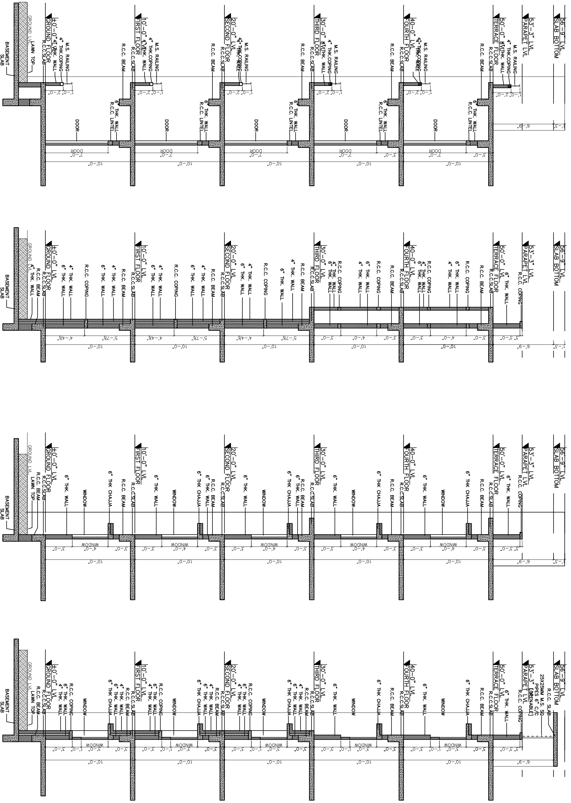
SECTION @ 07
