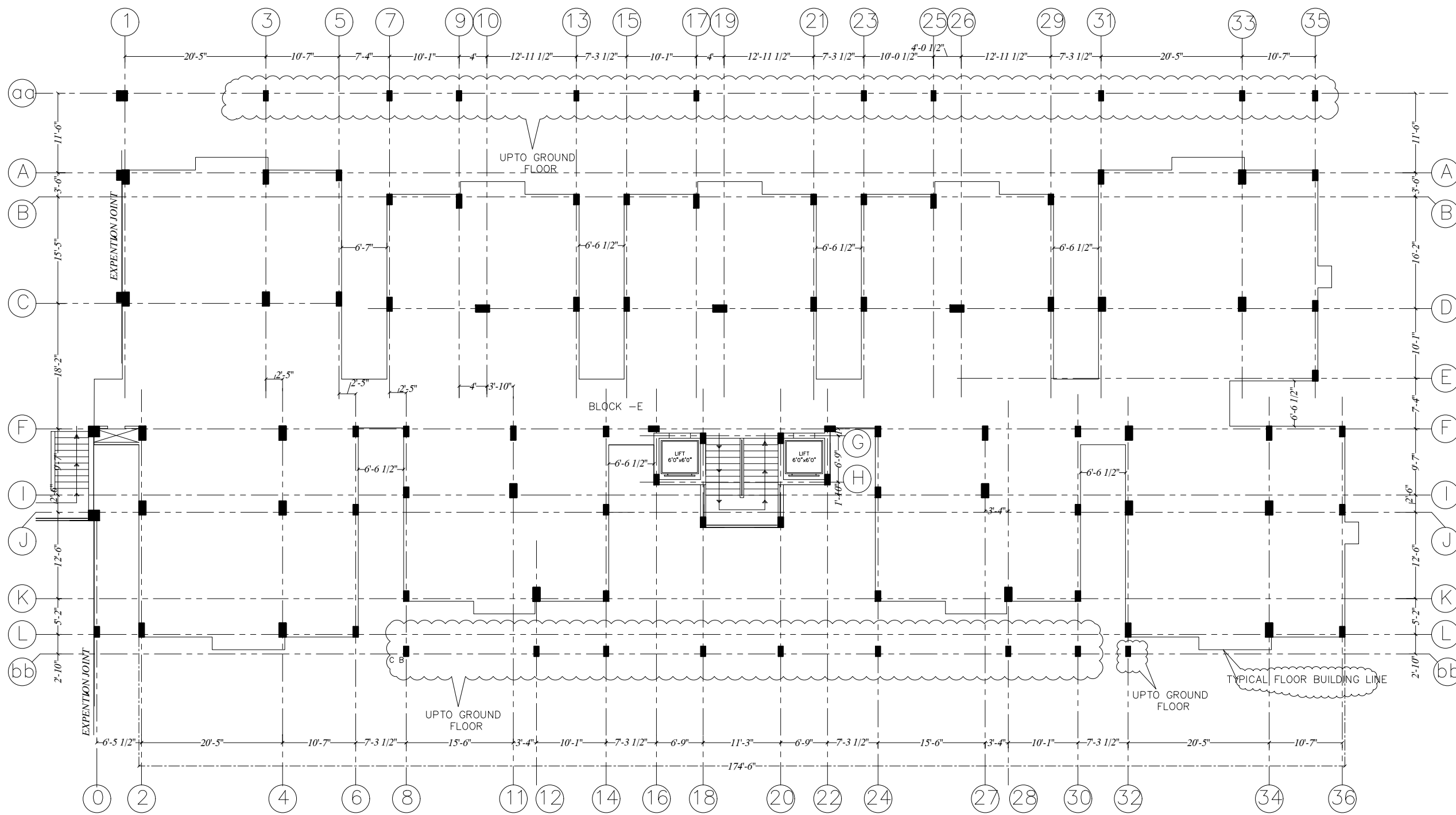
CENTER LINE DIAGRAM BLOCK - E
