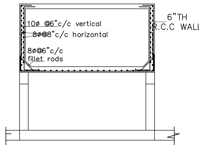
TYPICAL R.C.C. DETAILS
