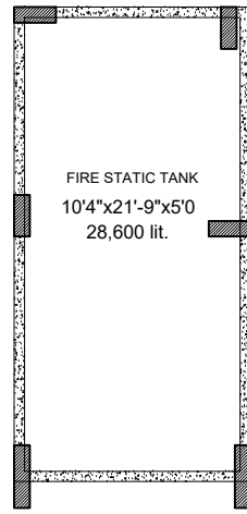
PLAN
