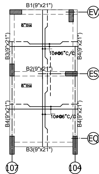
BOTTOM SLAB
