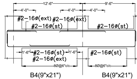
B4(9"x21") B4(9"x21")
