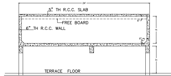
SECTION (X-X)
