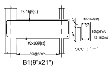
B1(9"x21")
