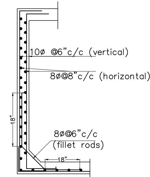
R.C.C WALL DETAILS
