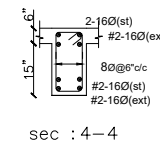
sec : 4-4
