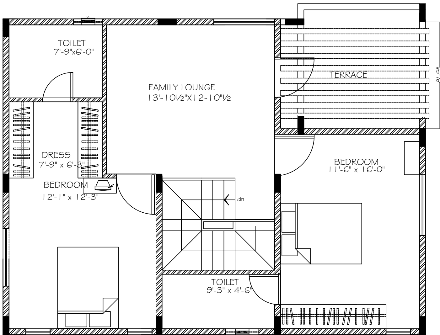
FIRST FLOOR
