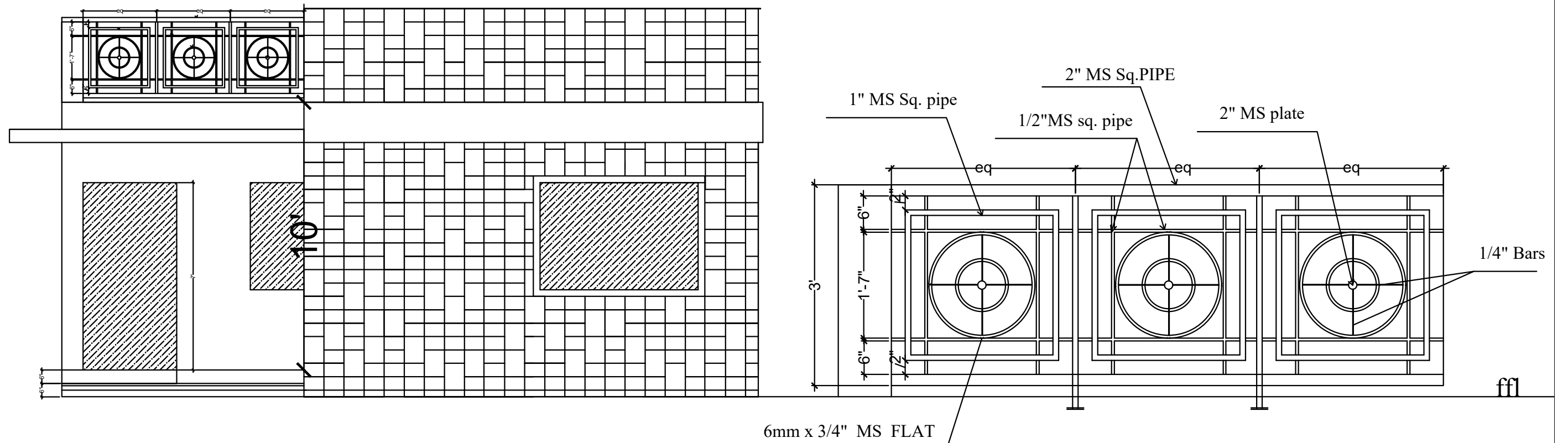
TYPE - A, B (single floor) ELEVATION
