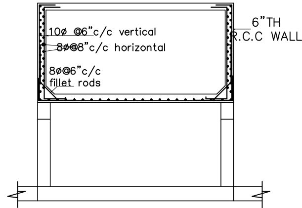
TYPICAL R.C.C. DETAILS
