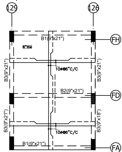
BOTTOM SLAB
