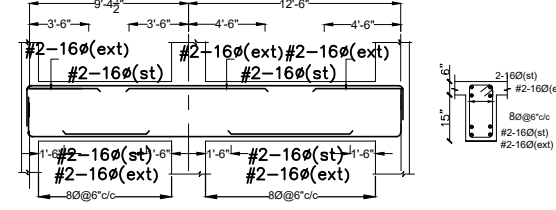
B3(9"x21")
