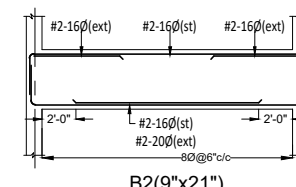
B2(9"x21")
