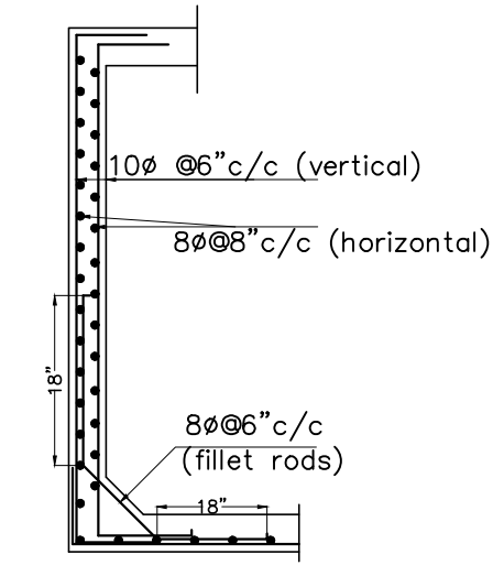
R.C.C WALL DETAILS
