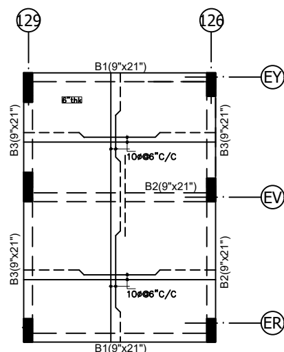
BOTTOM SLAB
