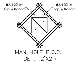
TYPICAL R.C.C. DETAILS
