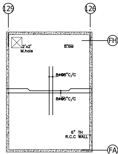
TOP SLAB
