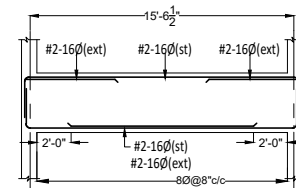
B1(9"x21")
