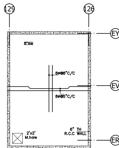
TOP SLAB
