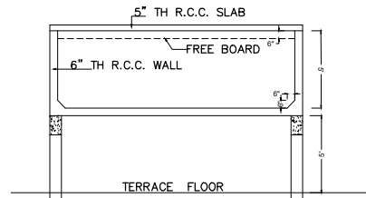
SECTION (X-X)
