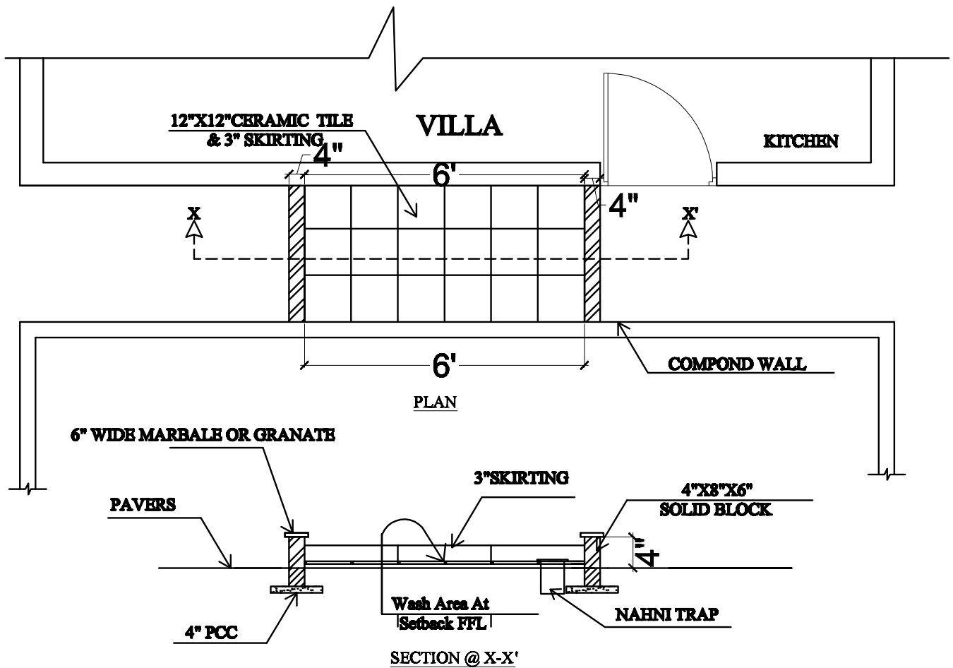
DETAIL@ A
