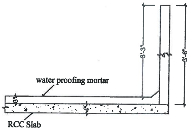
PARAPET WALL
