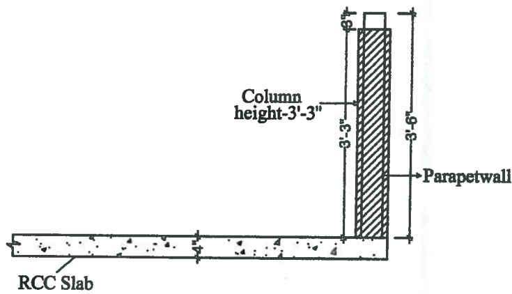
PARAPET WALL
