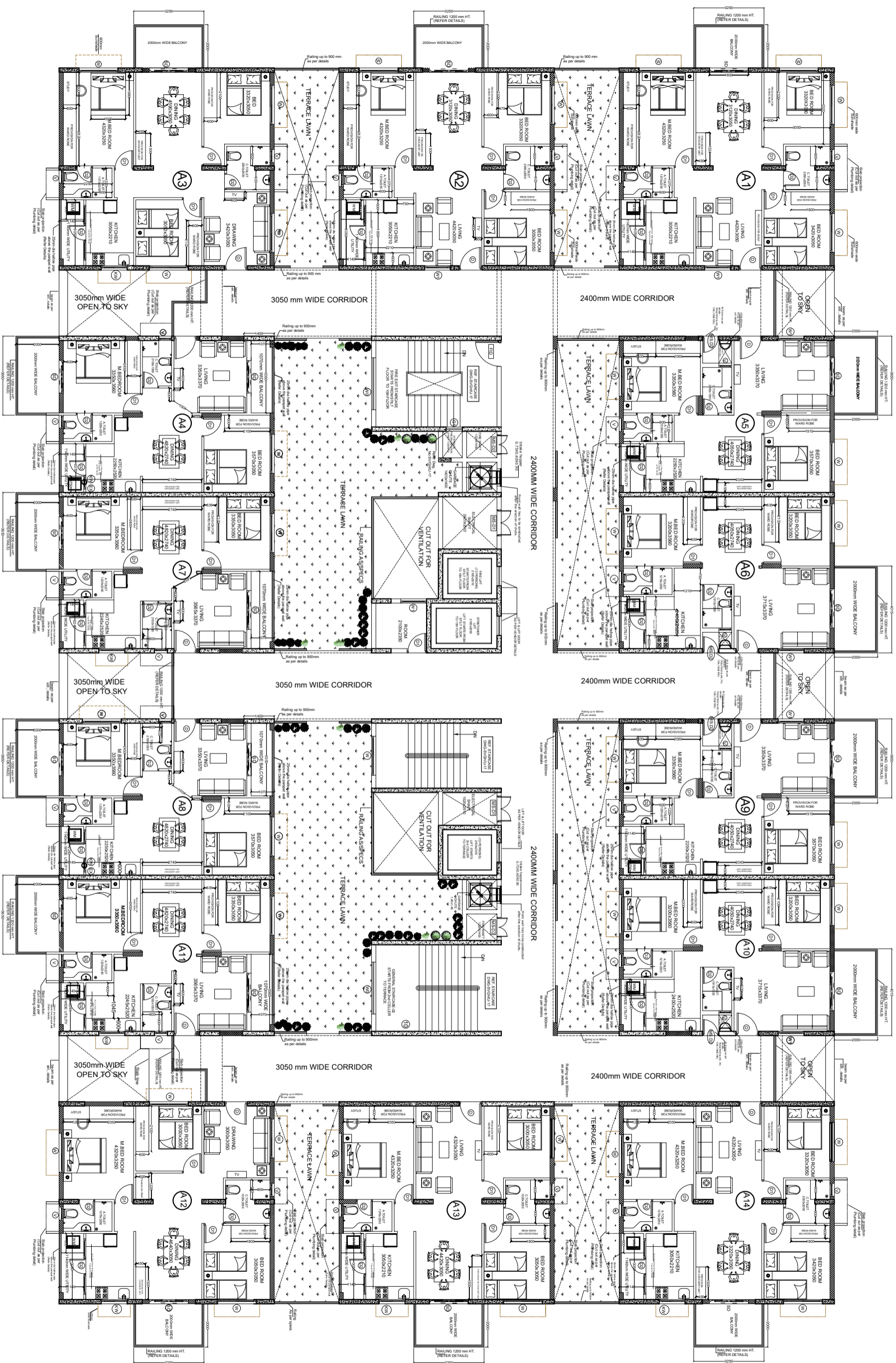
2ND TO 15TH TYPICAL FLOOR PLAN (ATRI BLOCK-A)
