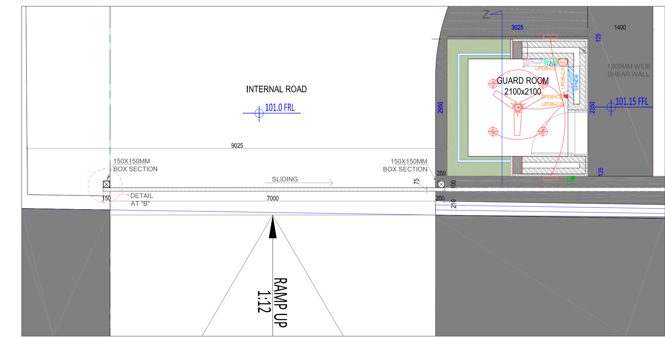
ELECTRICAL PLAN -2 (MATERIAL ENTRY GATE) SCALE- 1: 25
