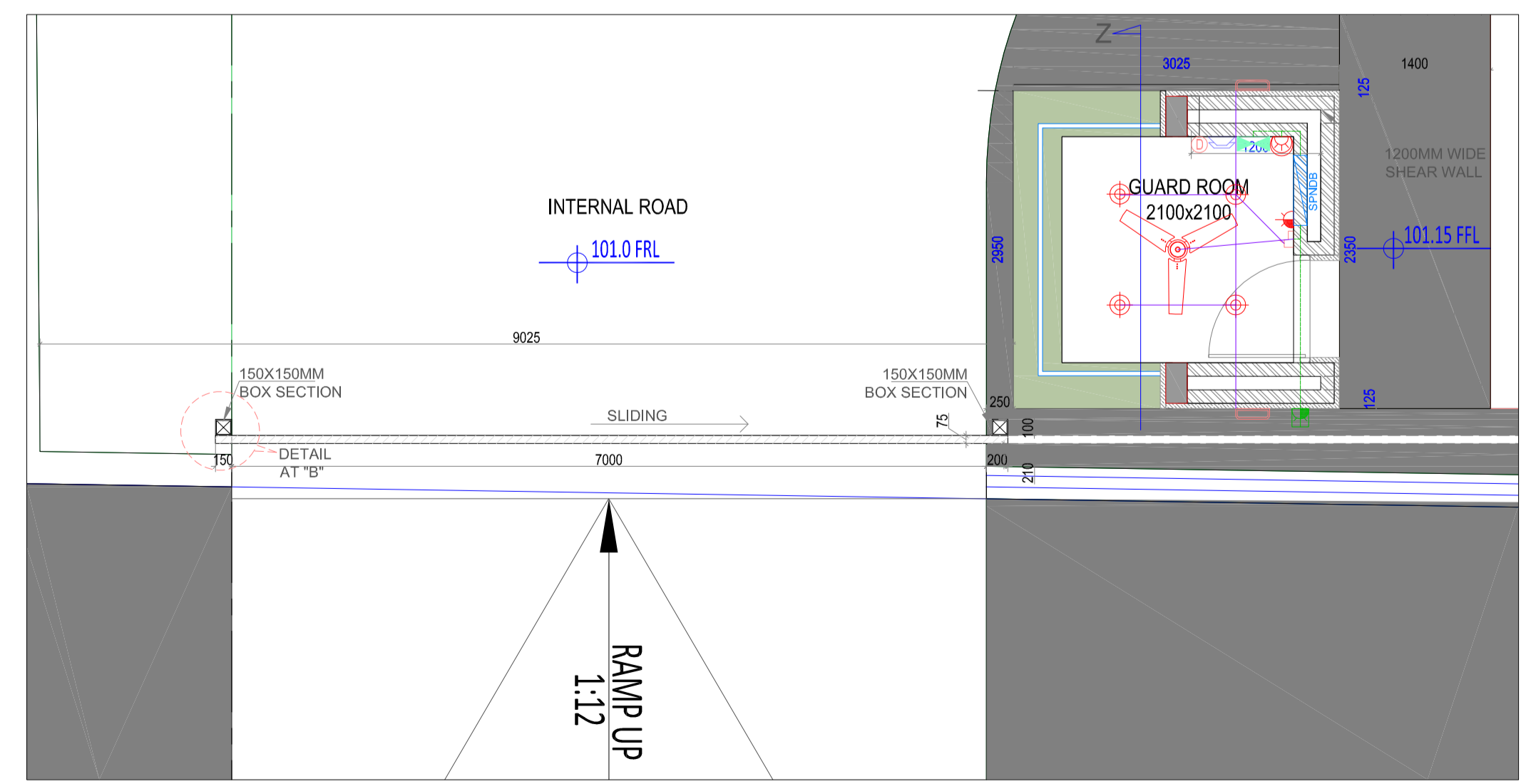
ELECTRICAL CONDUIT PLAN -2 (MATERIAL ENTRY GATE) SCALE- 1: 25
