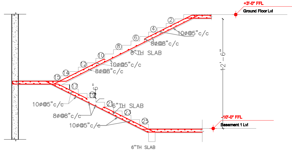
SECTION B-B
