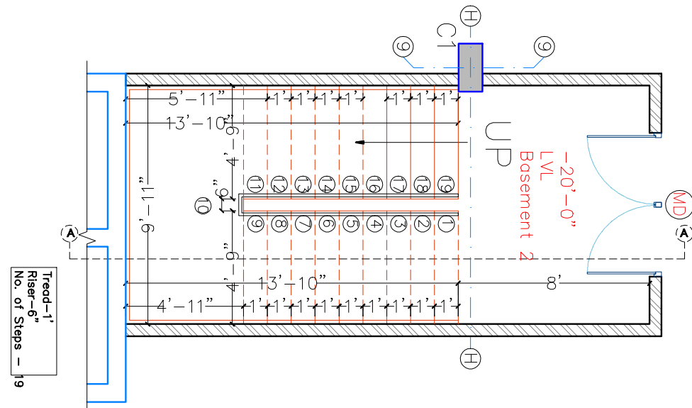
Plan at Basement 2 Lvl.
