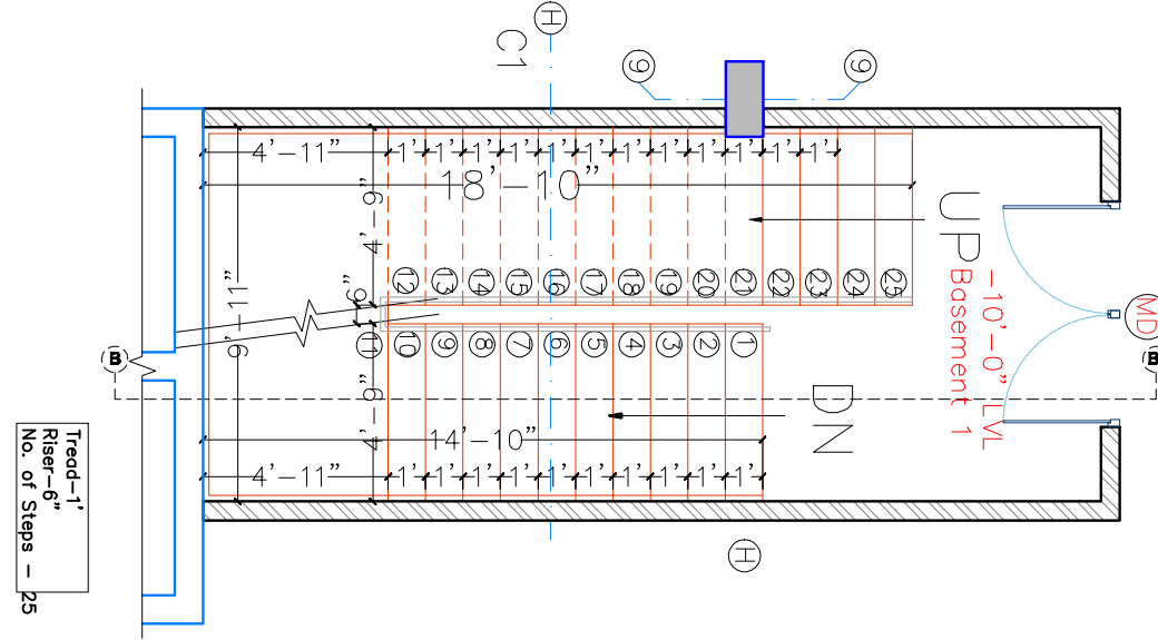
Plan at Basement 1 Lvl.
