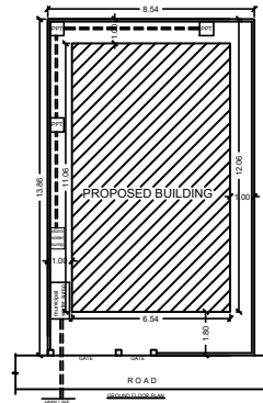
SITE PLAN-II
