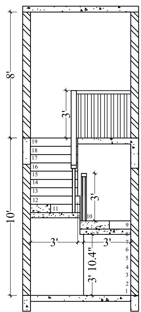
SECTION @ BB'
