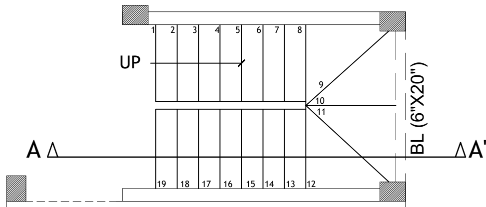
STAIRCASE PLAN
