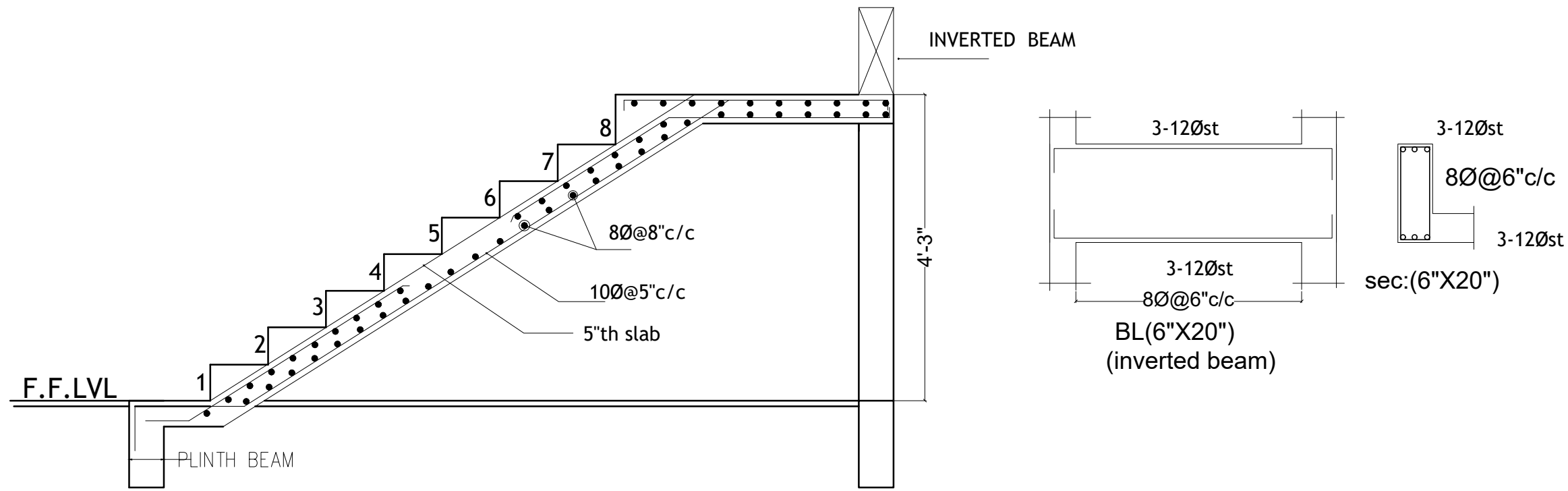
R.C.C SECTION DETAILS
