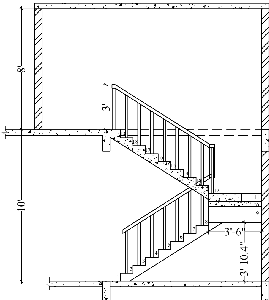
SECTION @ AA'
