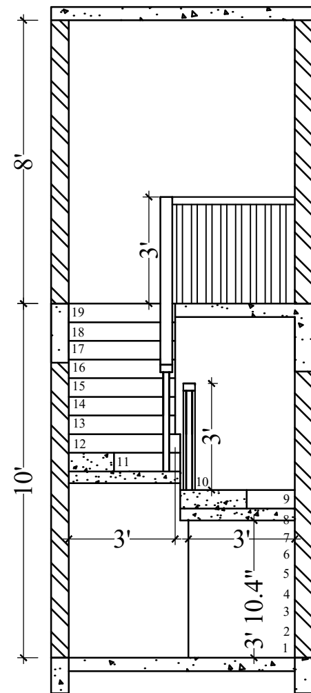
SECTION @ BB'
