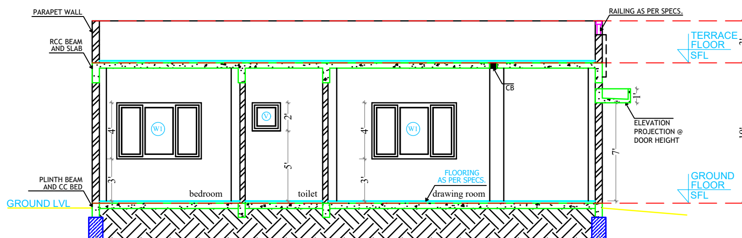
SECTION @ BB'
