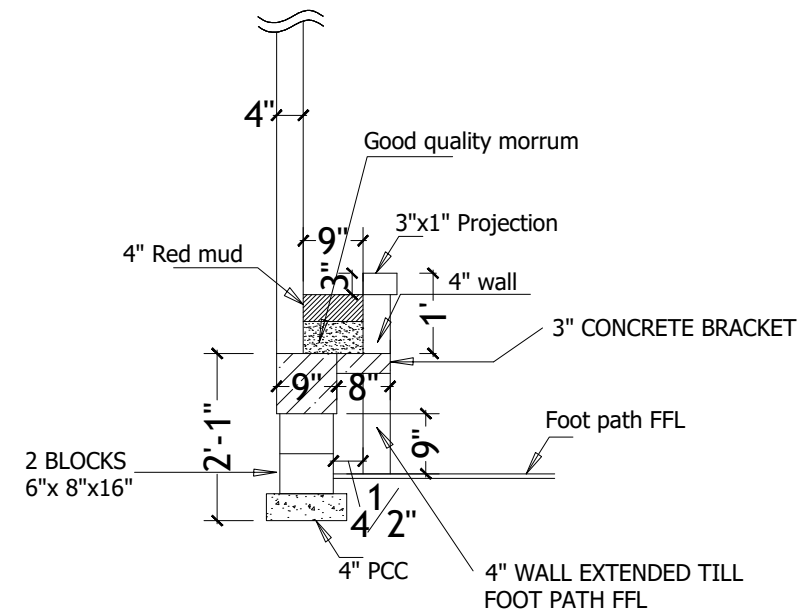
SECTION
