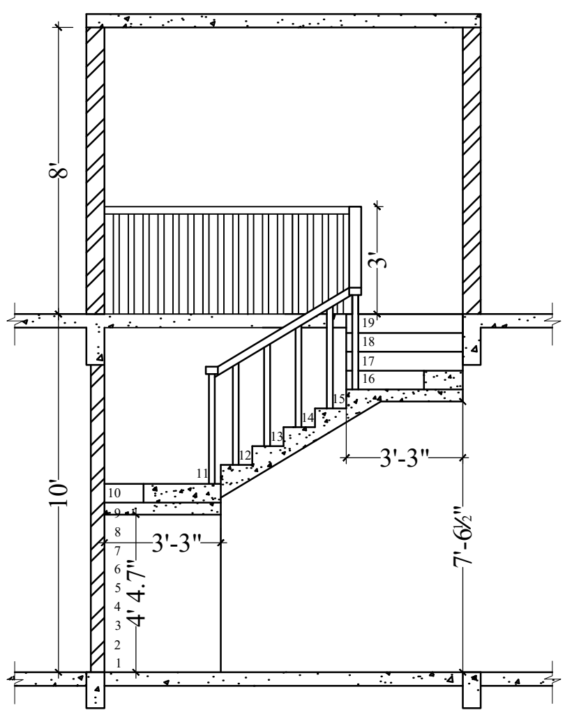
SECTION @ BB'
