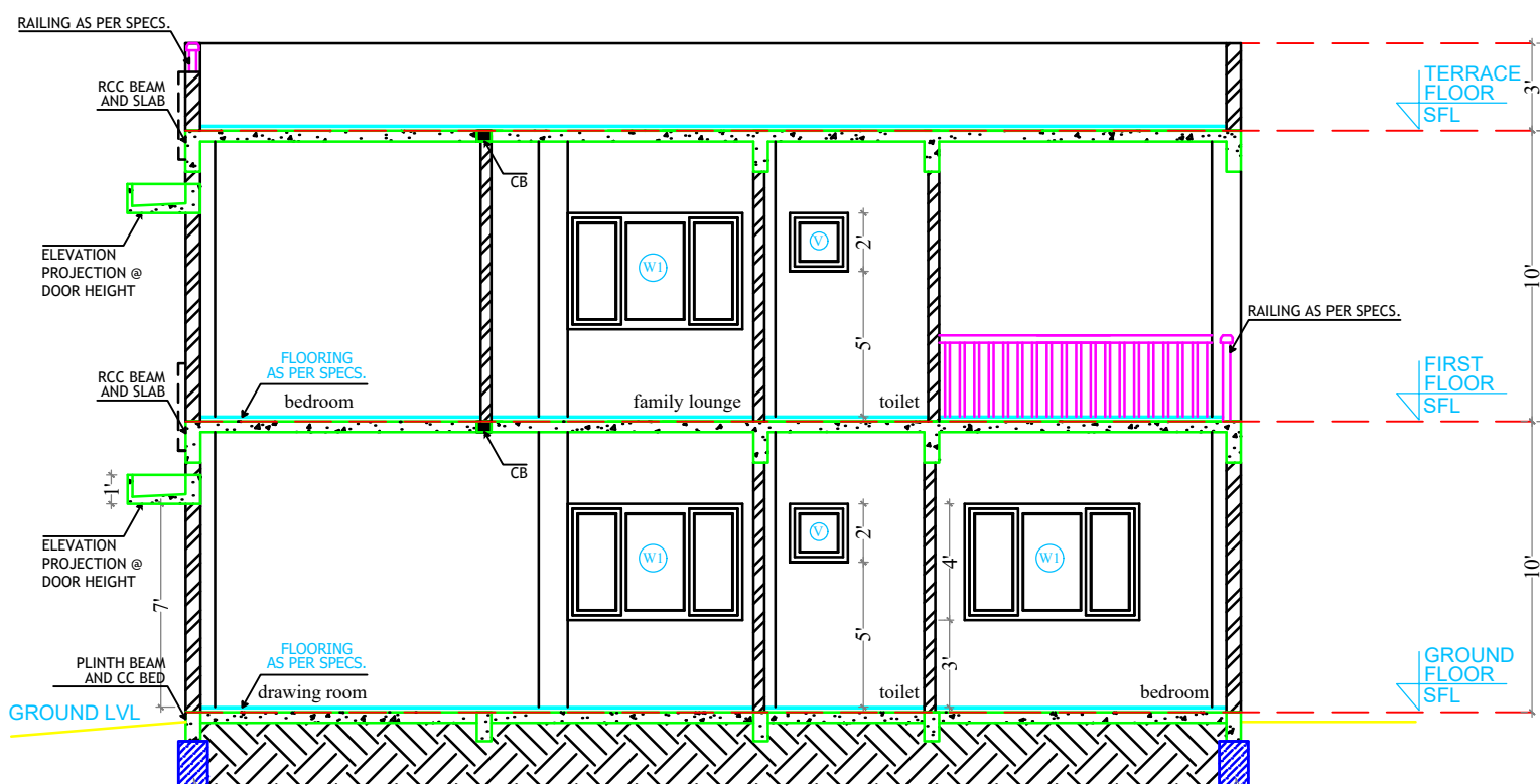
SECTION @ BB'
