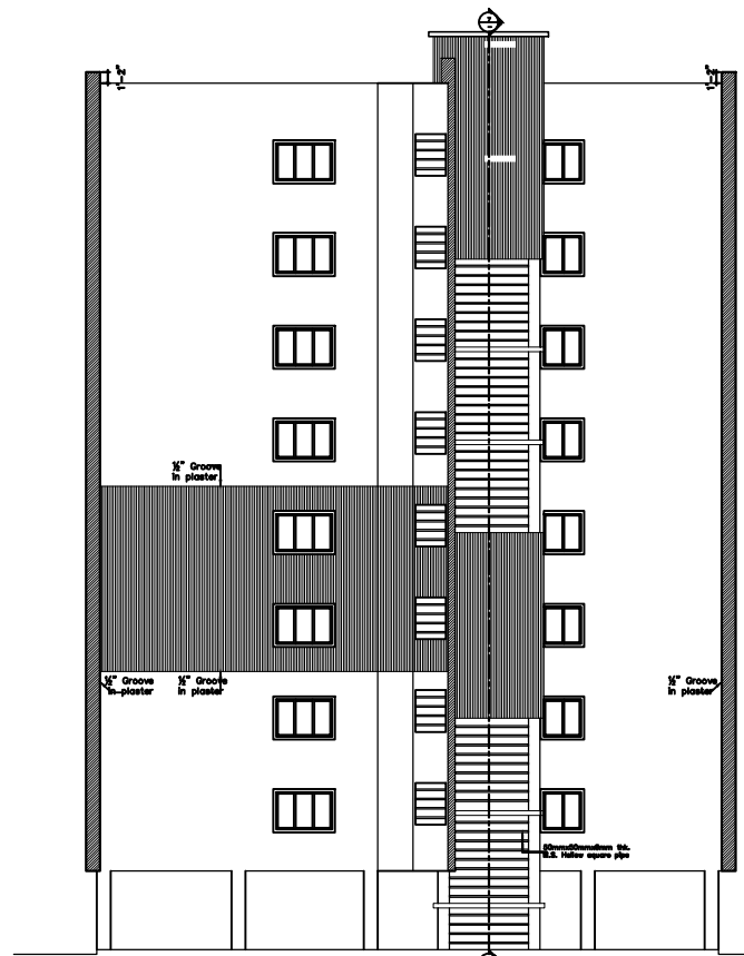
⑥ NORTH SIDE ELEVATION (© NORTH WEST CORNER)
