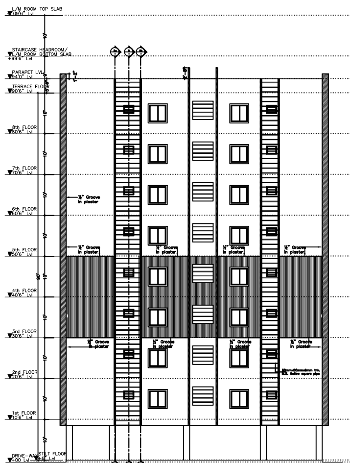
② NORTH SIDE ELEVATION (© NORTH EAST CORNER)
