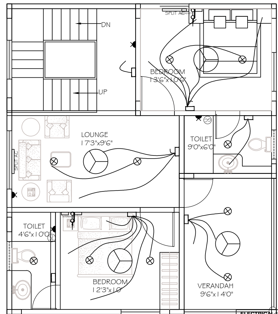
TYPICAL PLAN FOR FIRST & SECOND FLOOR
