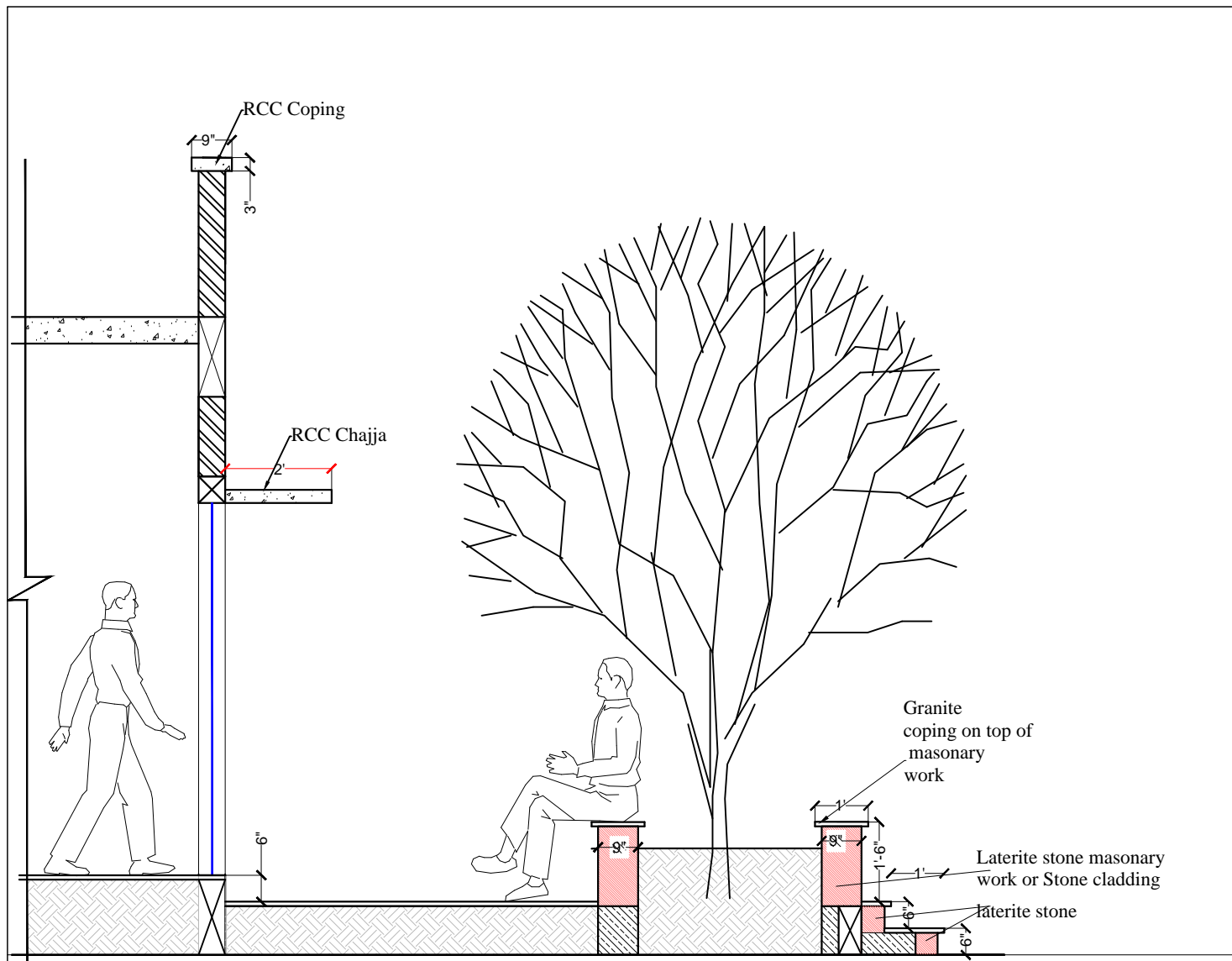
SECTION-VV
