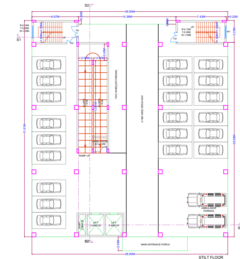
STILT FLOOR Scale-1:100
