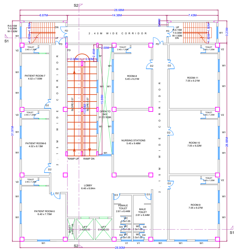
THIRD FLOOR Scale-1:100
