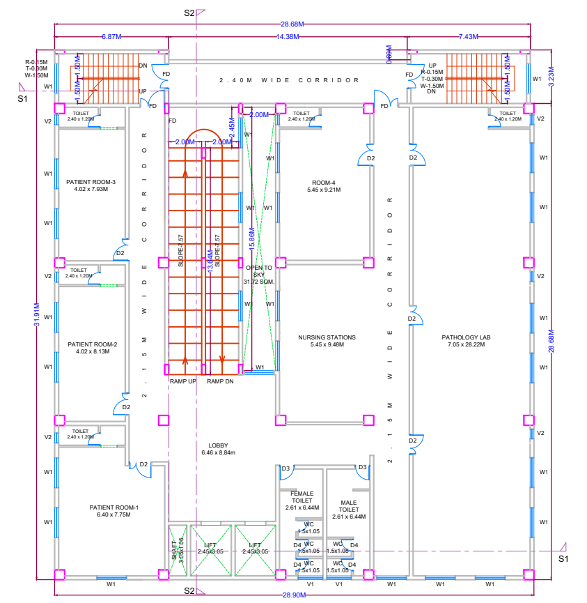
SECOND FLOOR Scale-1:100
