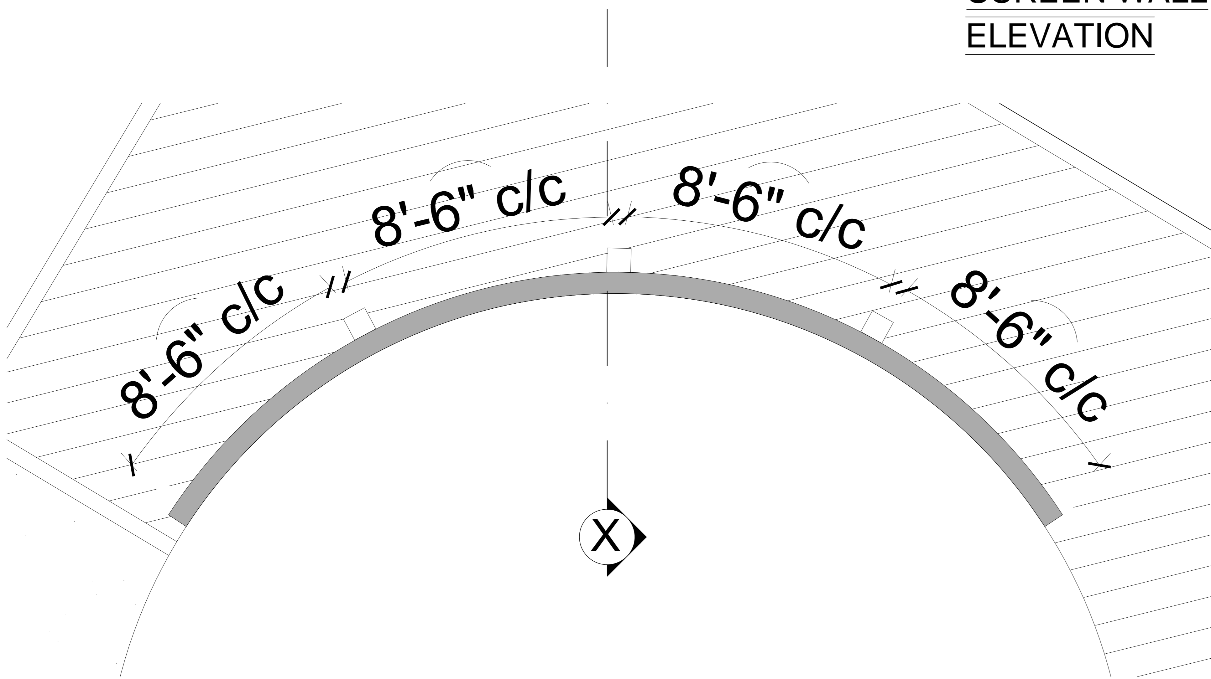
SCREEN WALL PLAN
