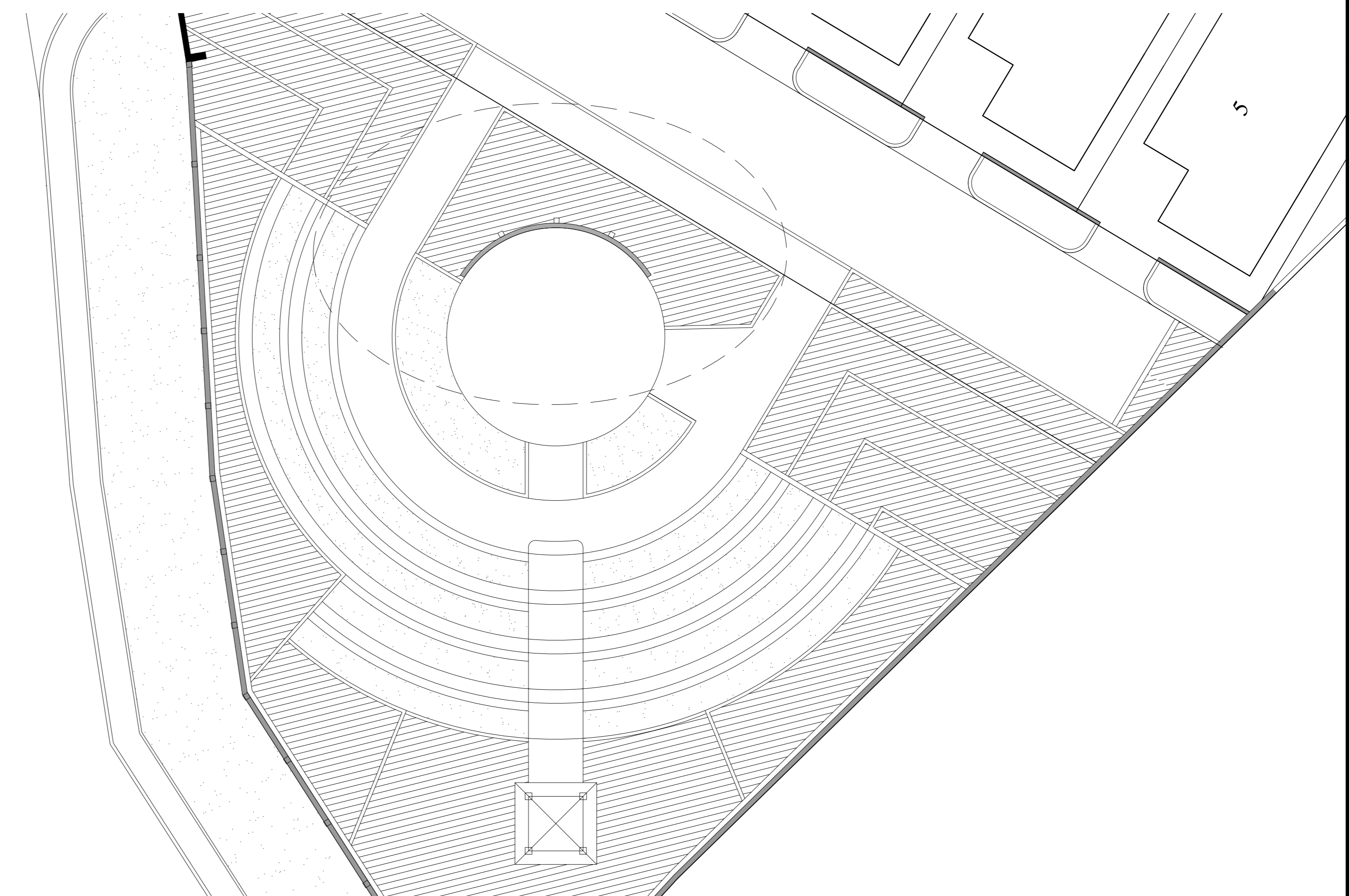
SCREEN WALL PLAN
