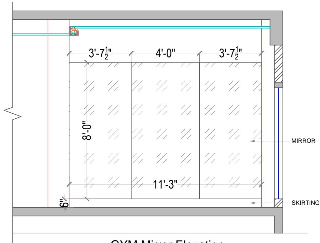
GYM Mirror Elevation Option 1
