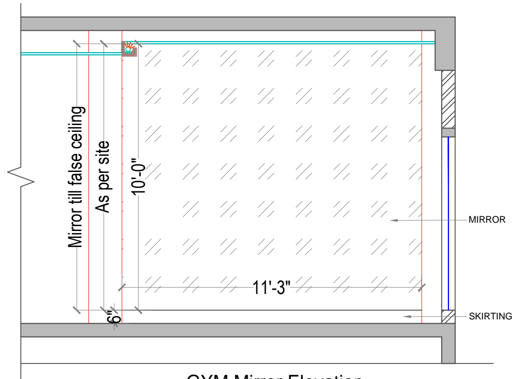
GYM Mirror Elevation Option 2
