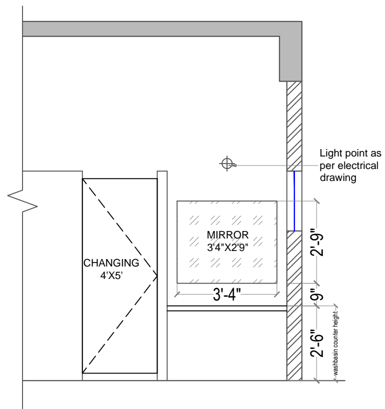
Wash Area Mirror Elevation
