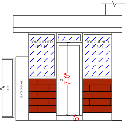
SIDE A ELEVATION
