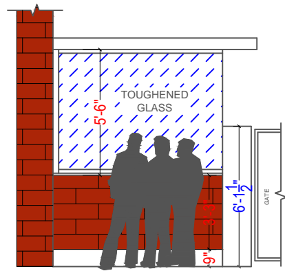
SIDE B ELEVATION
