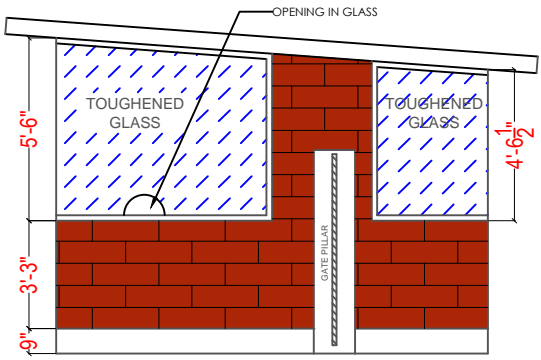
SIDE C ELEVATION
