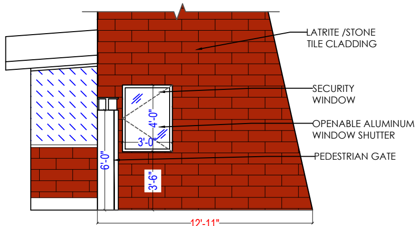
SIDE D ELEVATION
