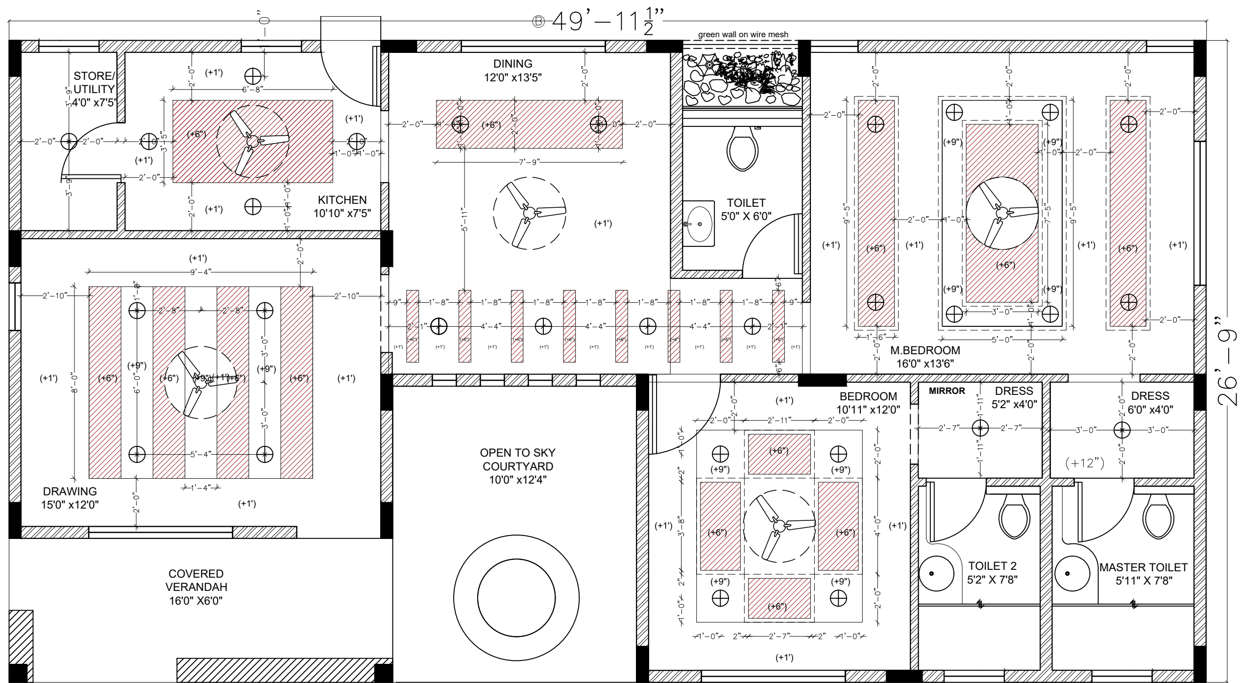
FARM HOUSE – 2BHK FALSE CEILING PLAN BUILT UP AREA = 1200 Sq.Ft.
