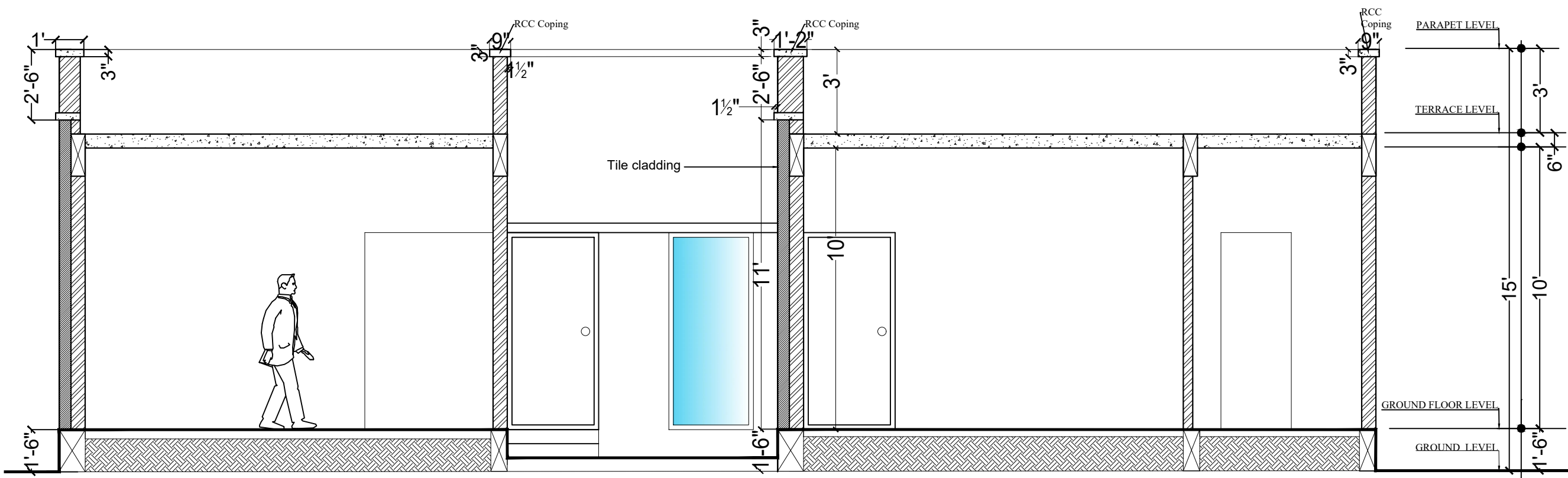
SECTION-XX
