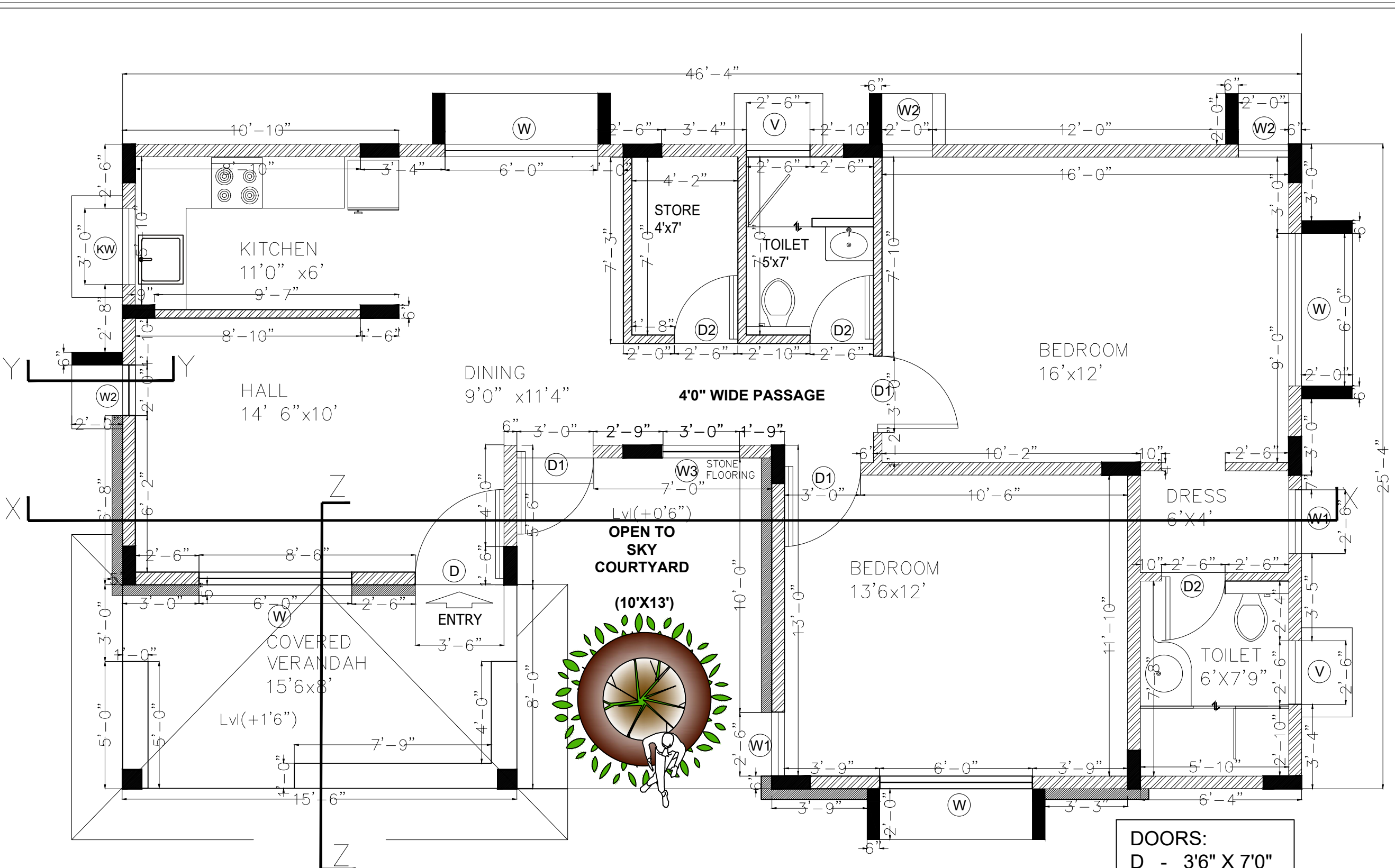
FARM HOUSE – 2BHK FLOOR PLAN BUILT UP AREA = 1044 Sq.Ft. {875 + 125 (Covered Verandah)}
