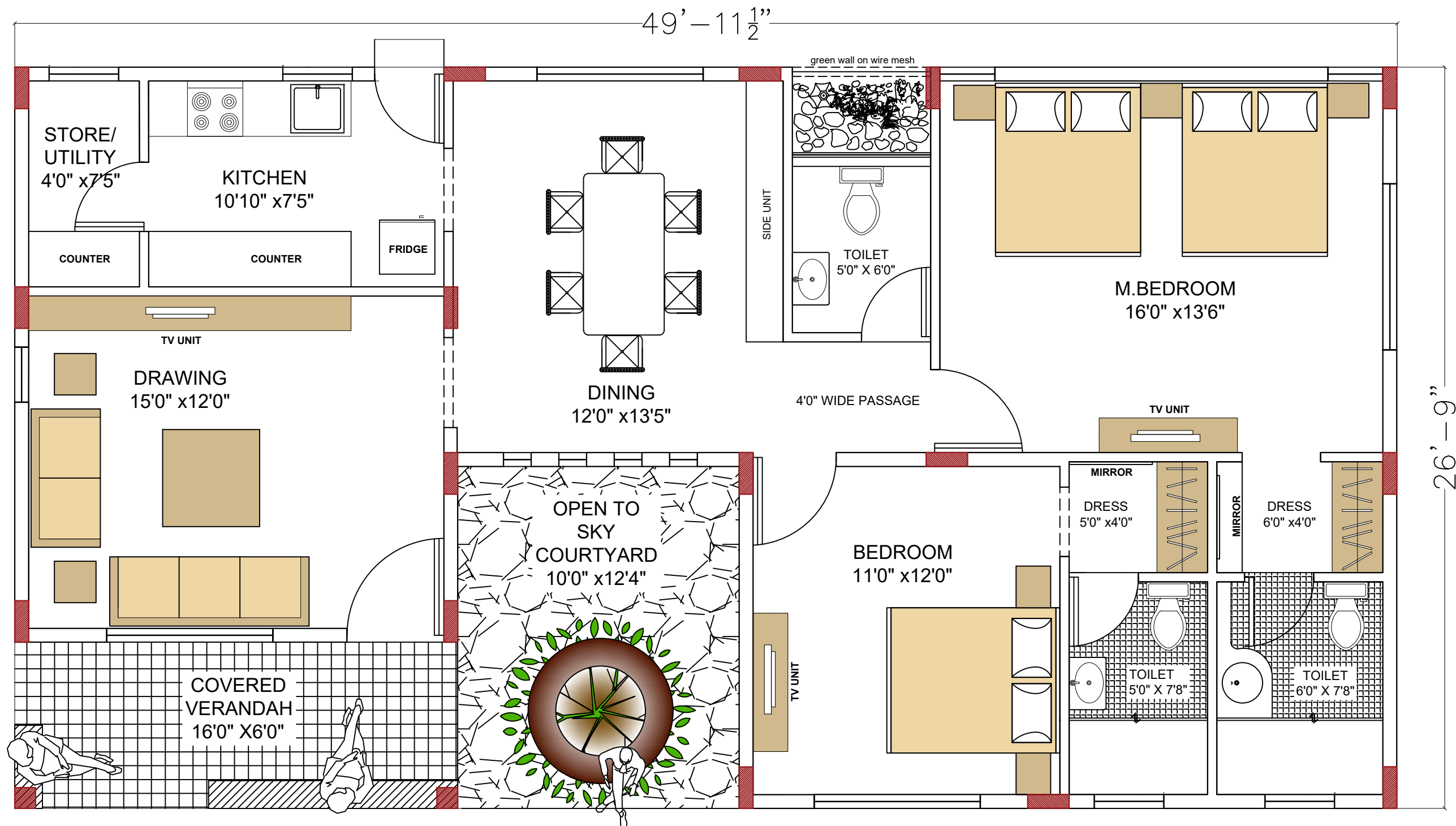
FARM HOUSE –2BHK FLOOR PLAN BUILT UP AREA = 1200 Sq.Ft.
