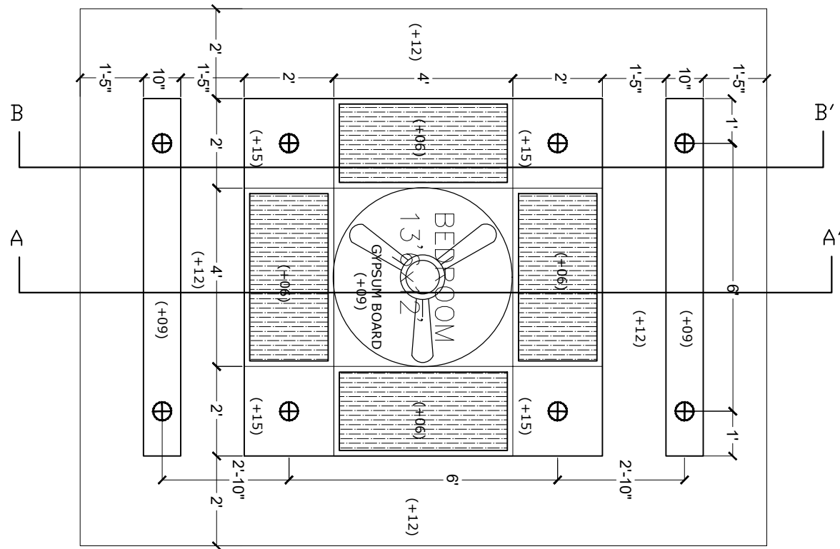
PLAN (room)
