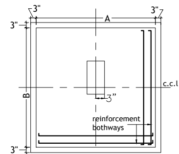
FOOTING DETAILS
