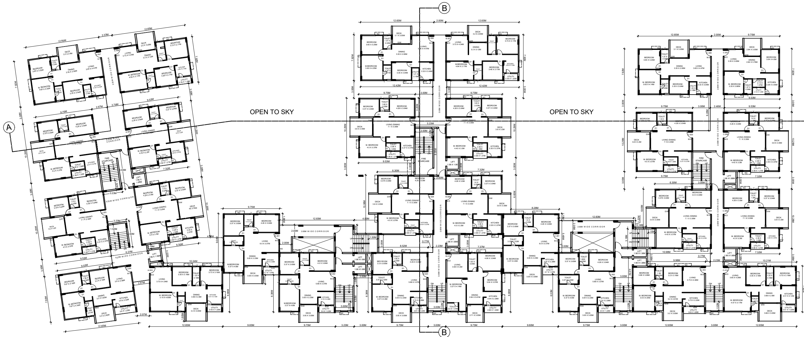
TYPICAL FLOOR PLAN (3RD TO 10TH FLOOR)
