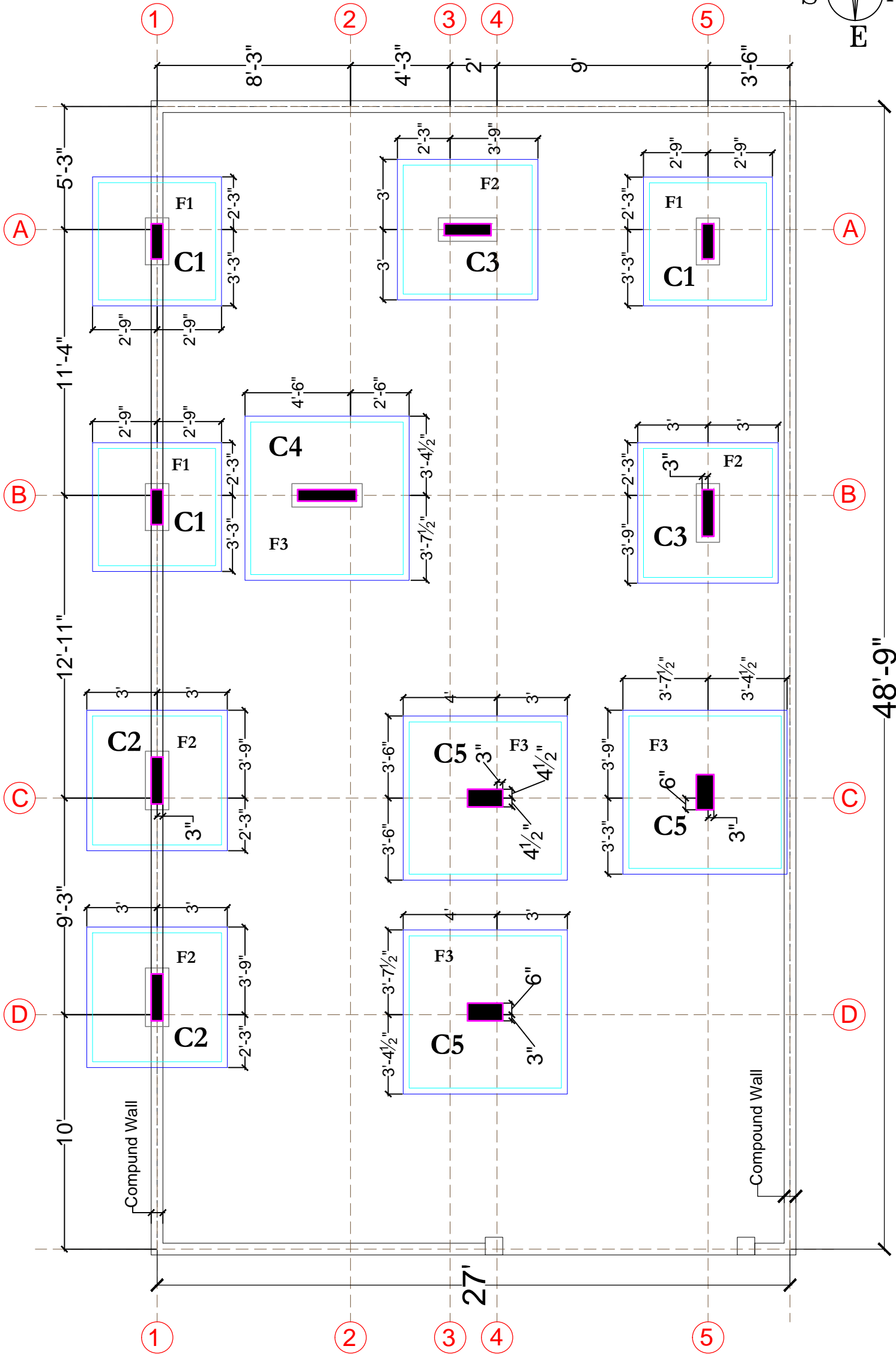
CENTRE LINE PLAN
