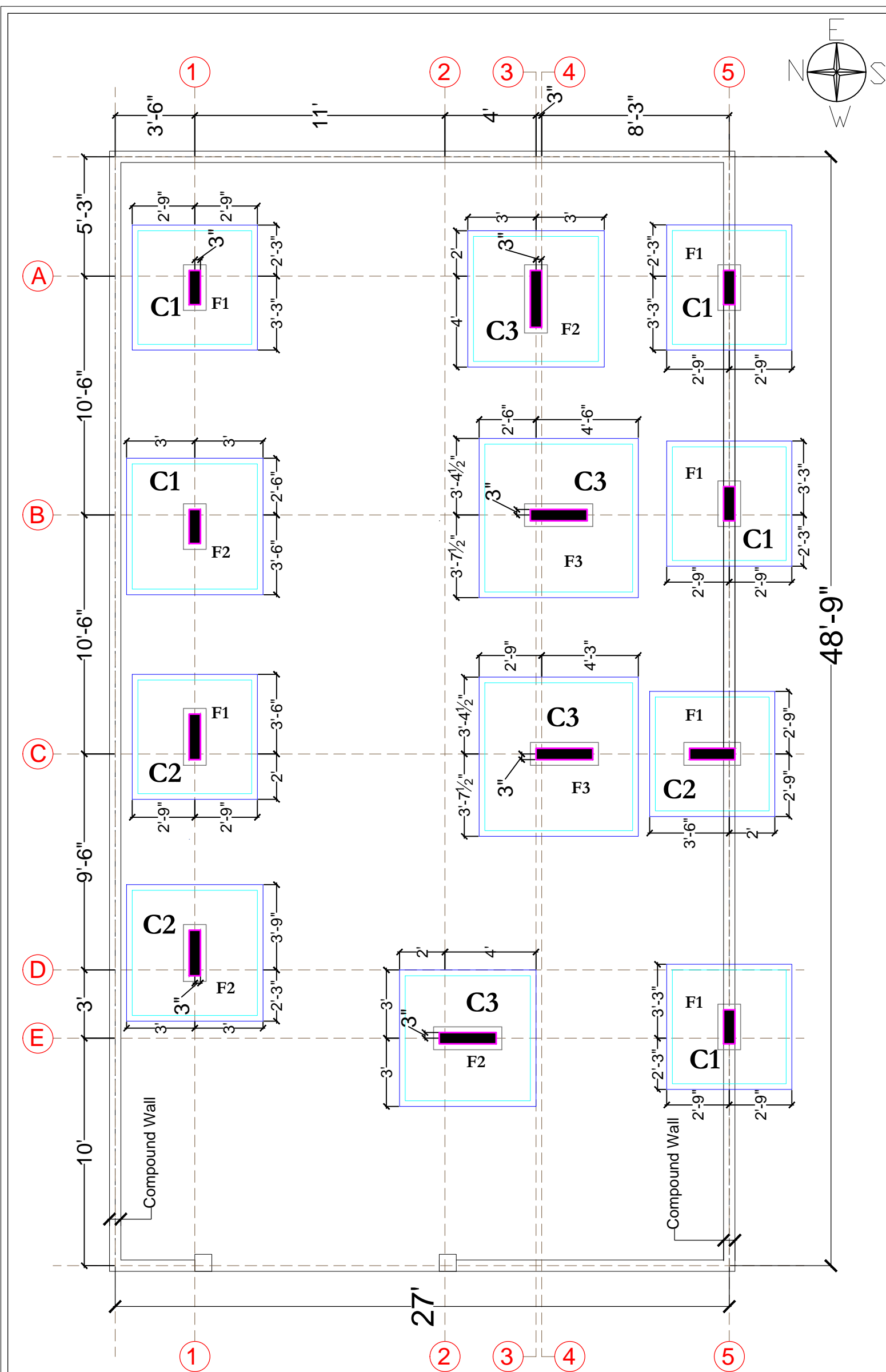
CENTRE LINE DRAWING
