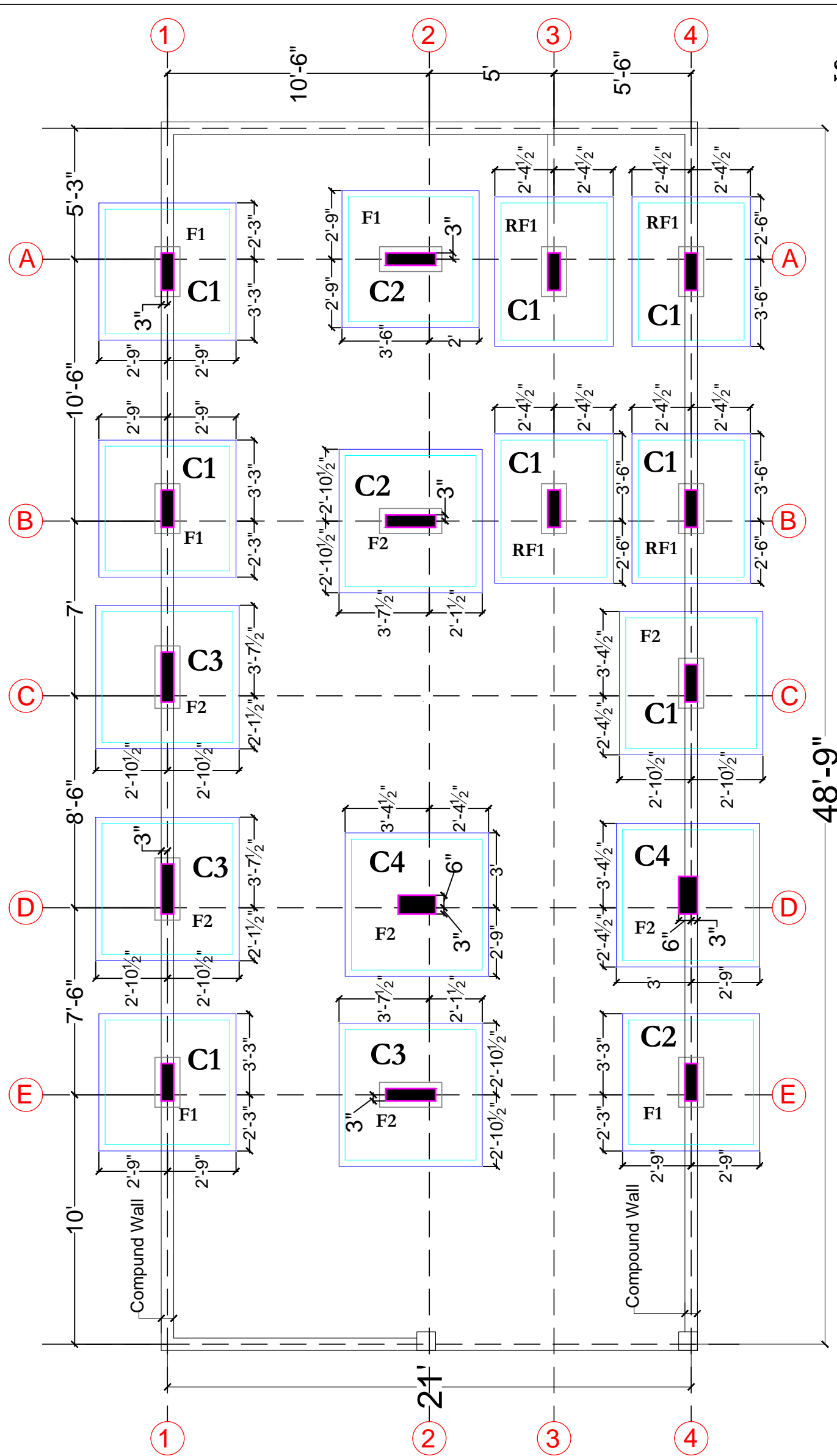
CENTRE LINE PLAN
