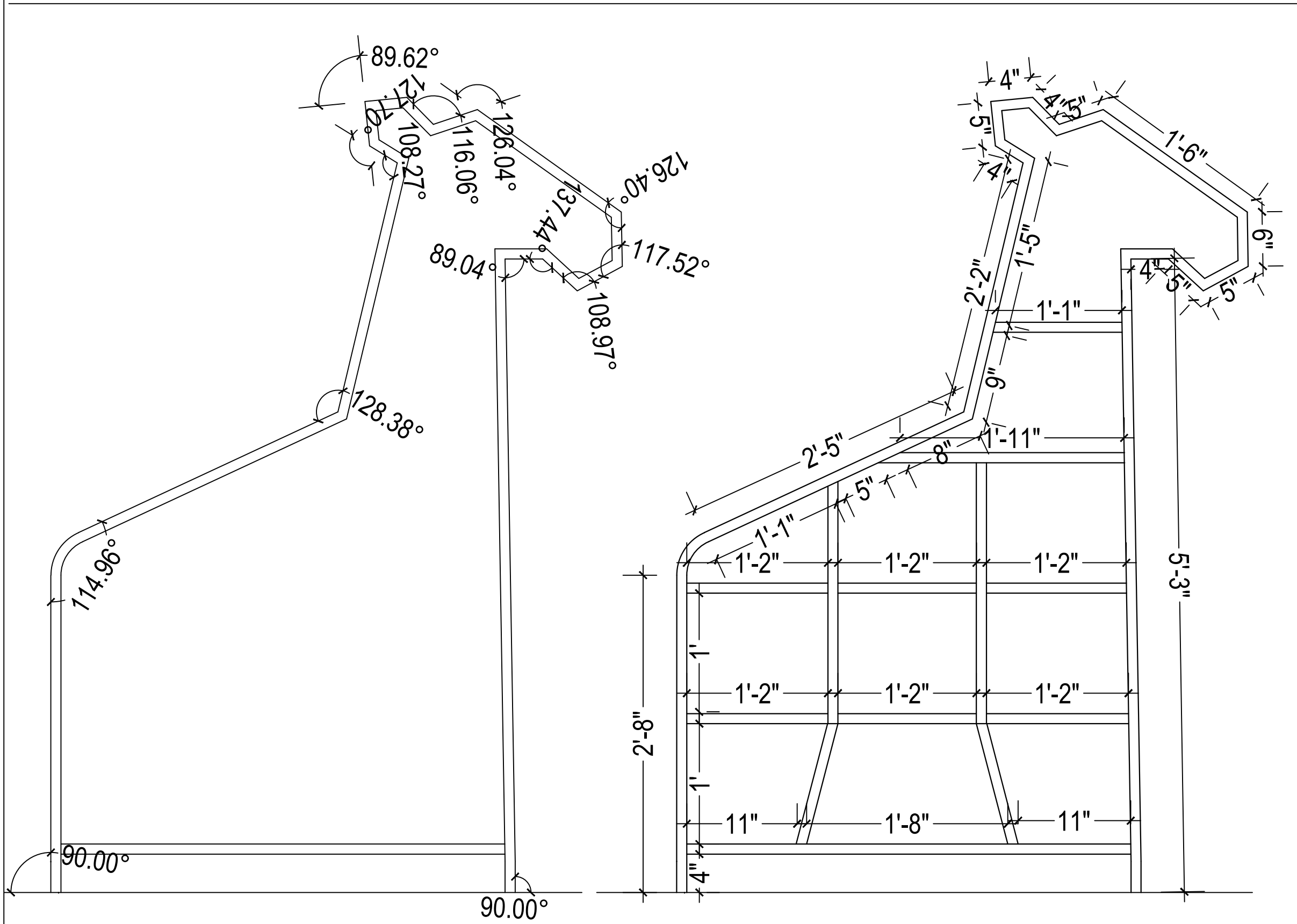
ANGULAR MEASUREMENT DETAILS
