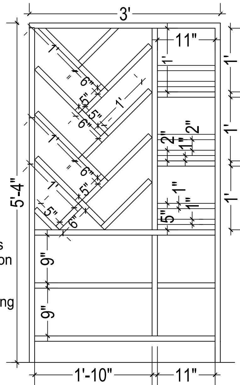
MEASUREMENT DETAIL CD7 FIRST FLOOR LIBRARY - STORAGE UNIT 3'-0" x 1'-3"
