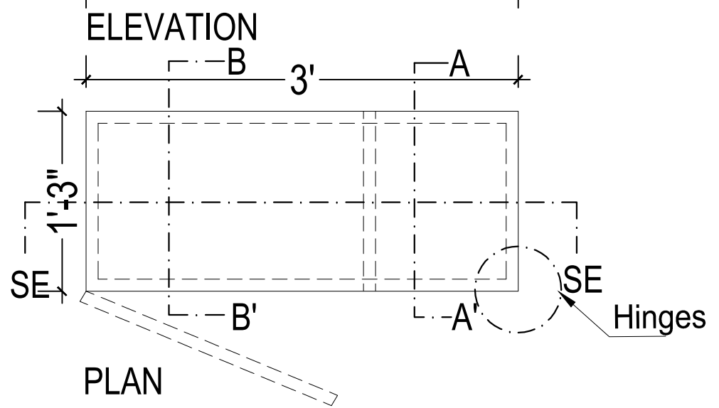
MEASUREMENT DETAIL CD7 FIRST FLOOR LIBRARY - STORAGE UNIT 3'-0" x 1'-3"
