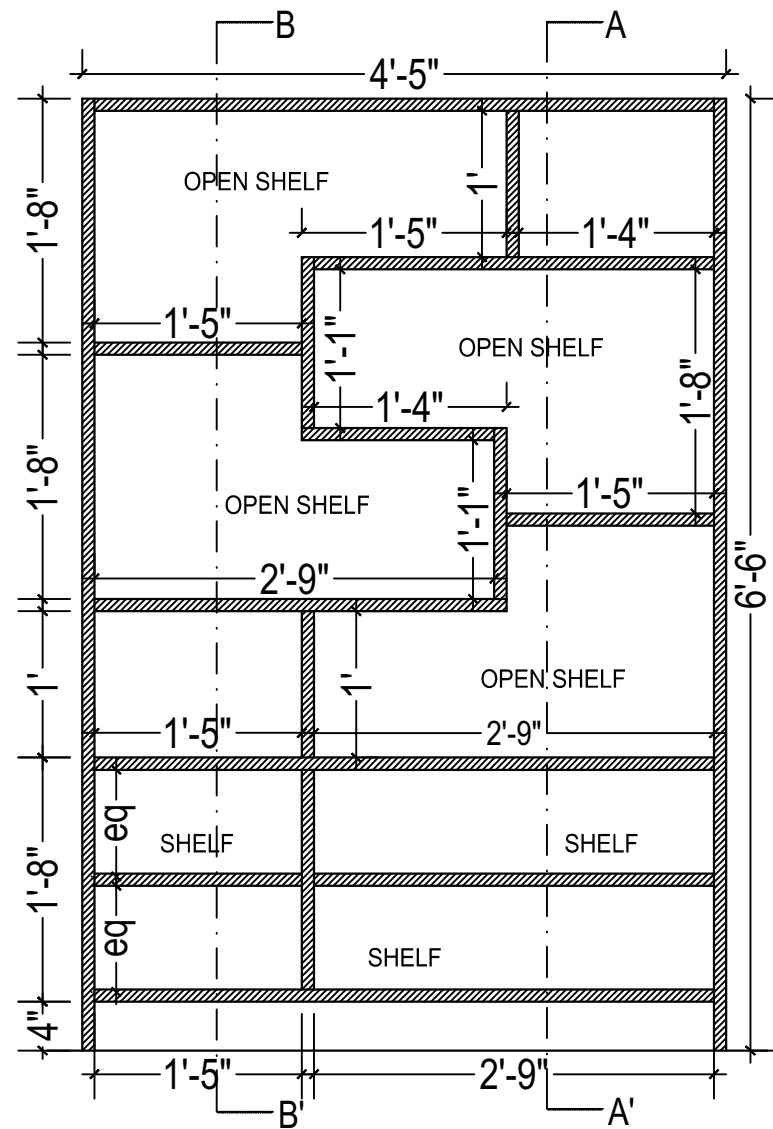
SECTIONAL ELEVATION
