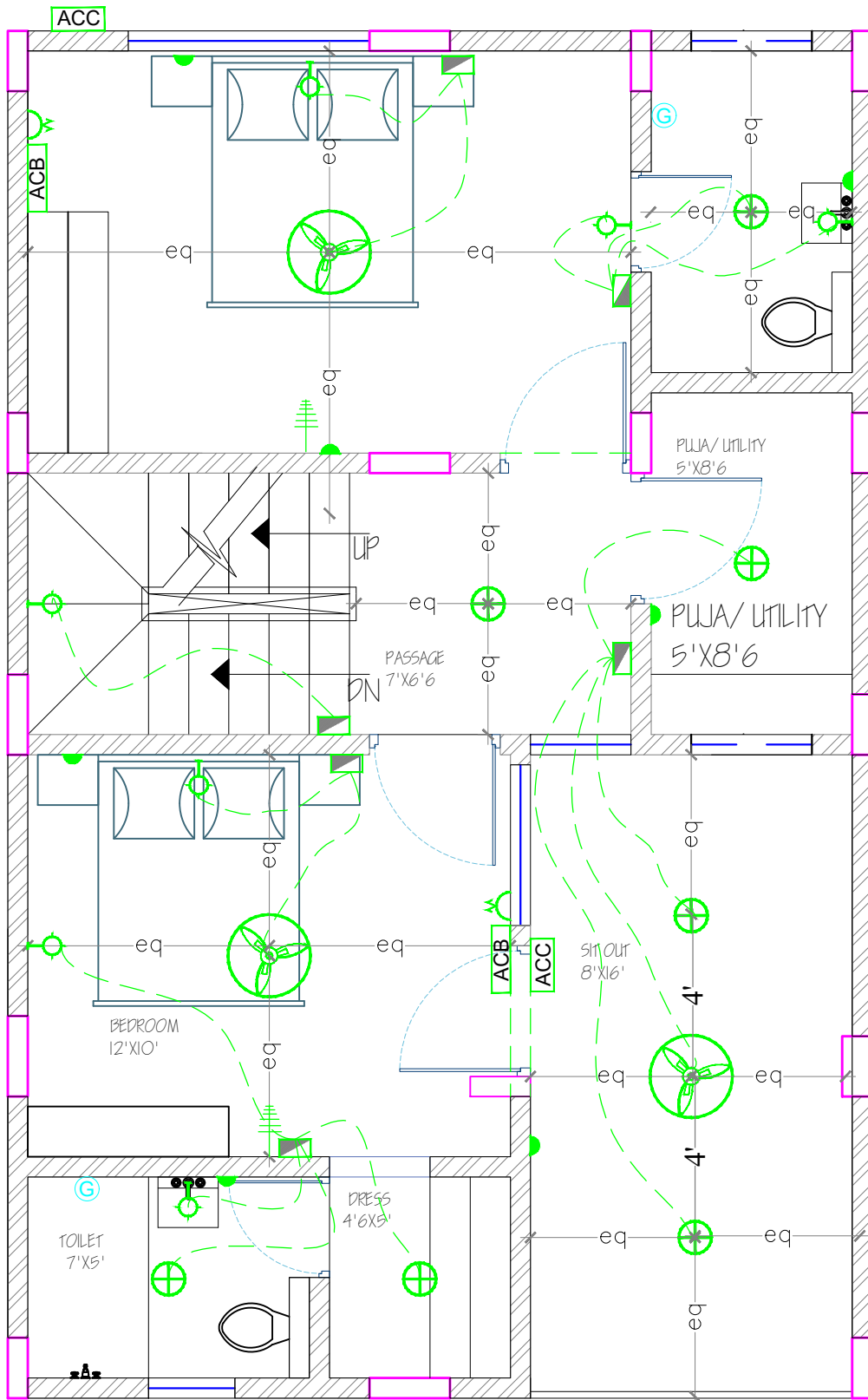
FIRST FLOOR
