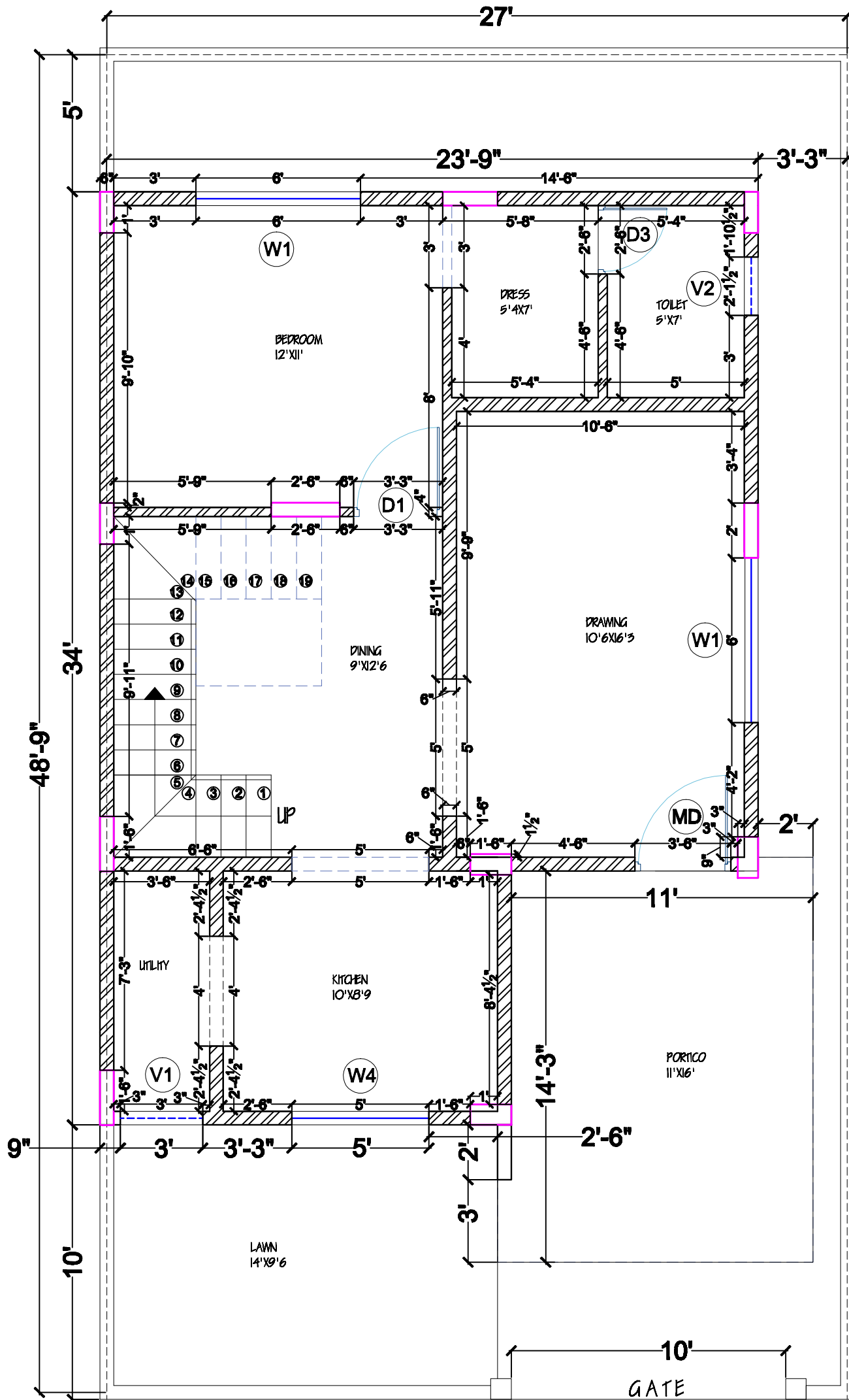
GROUND FLOOR
