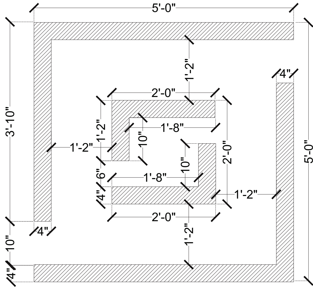
MEASUREMENT DETAILS OF STAIR CASE - 1
