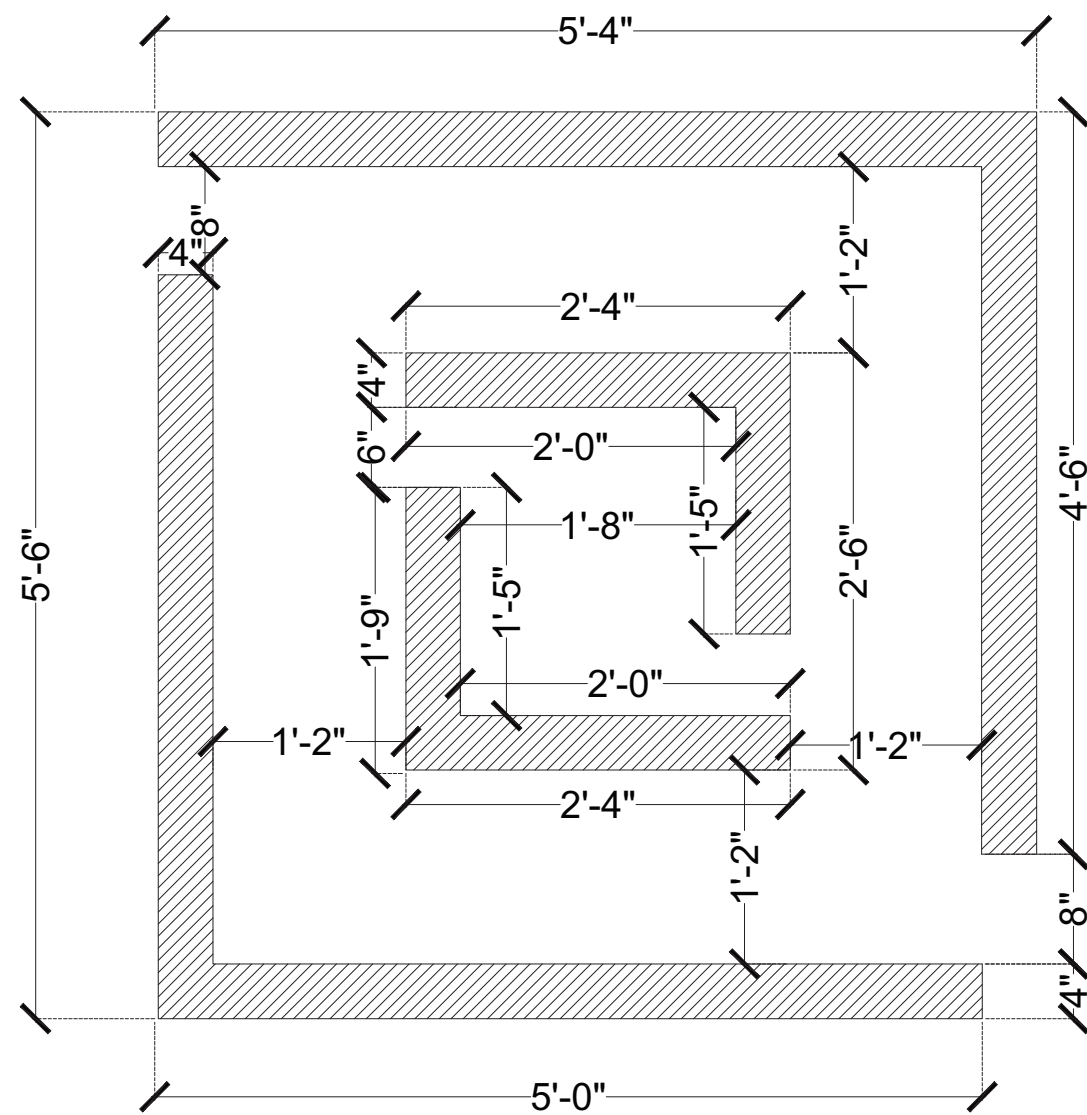
MEASUREMENT DETAILS OF STAIR CASE - 2
