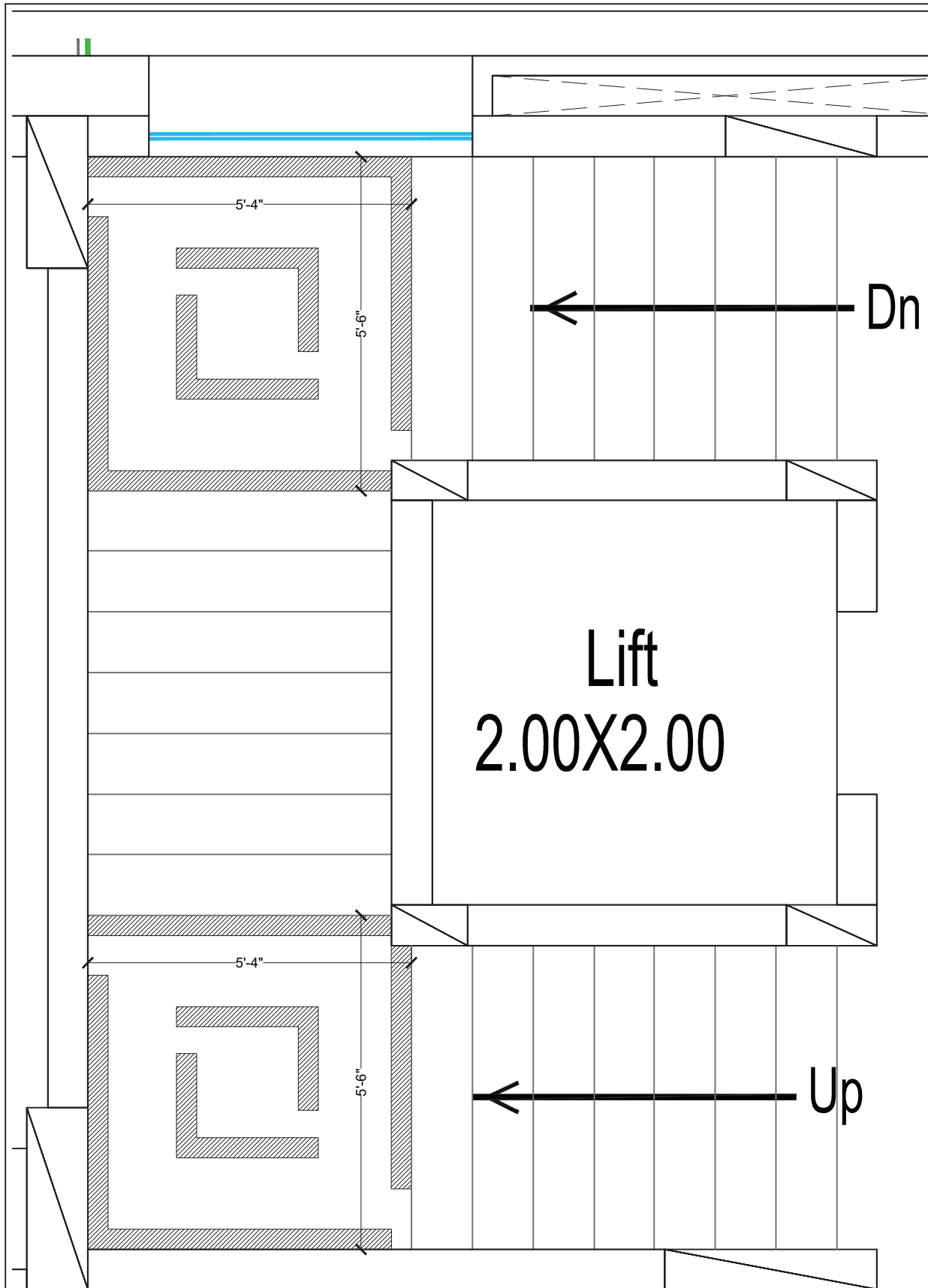
STAIR CASE - 2
