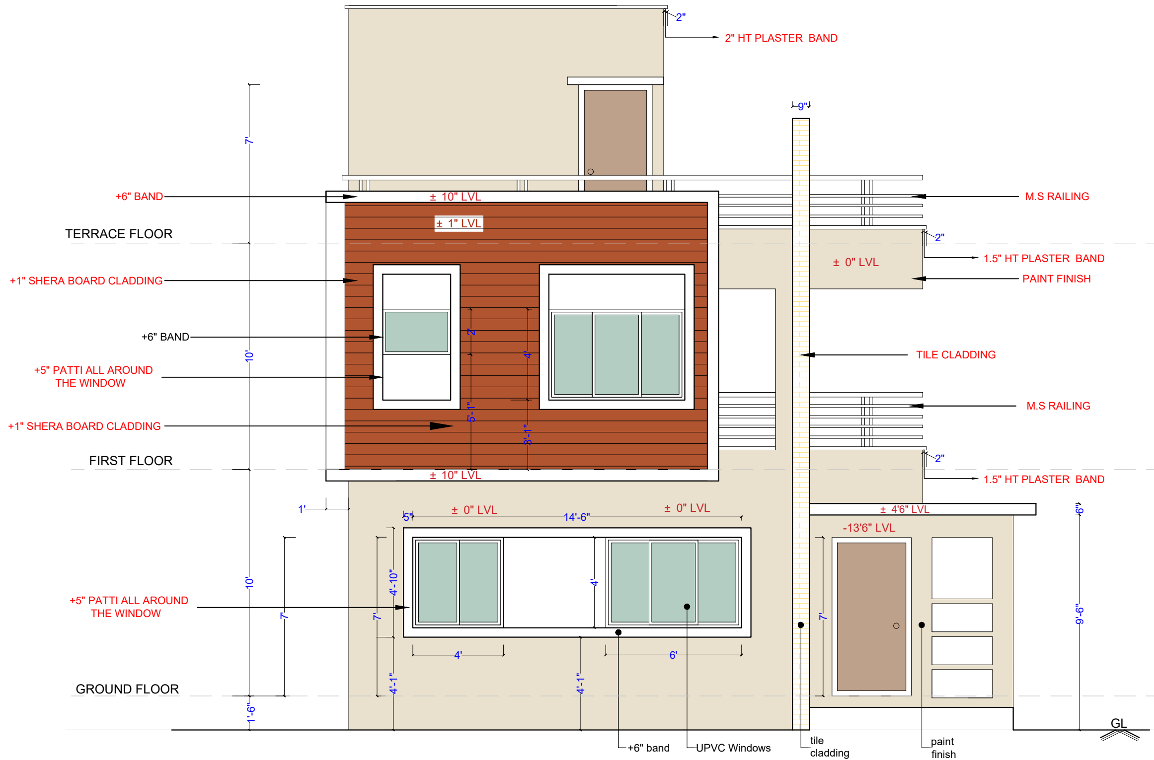
EAST ELEVATION
